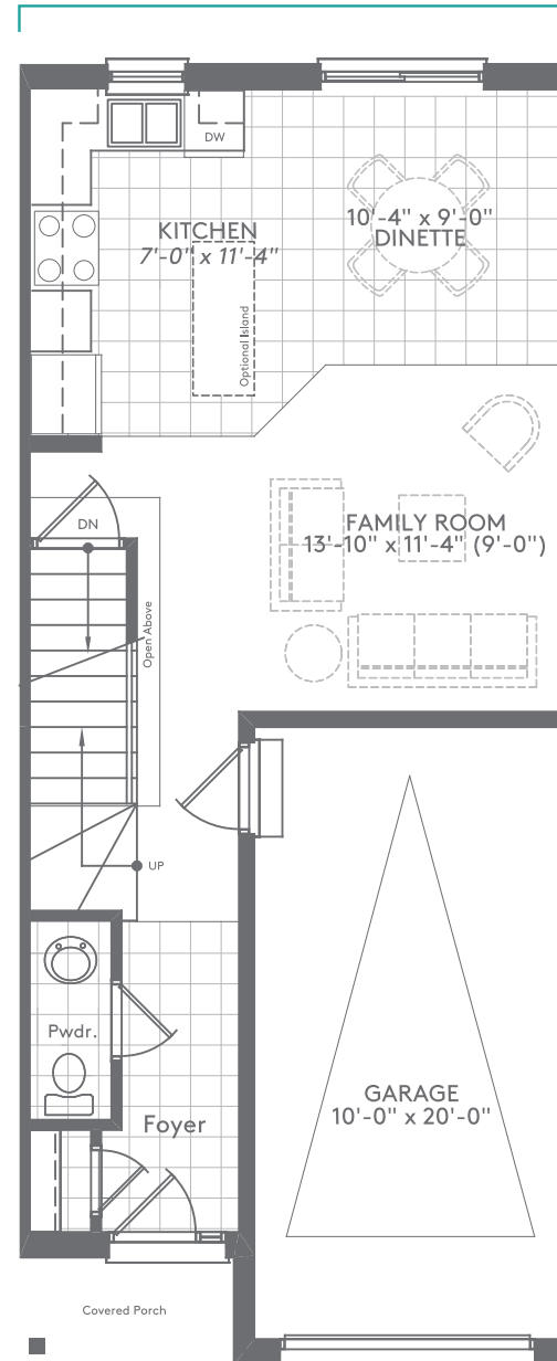
MAIN LEVEL
