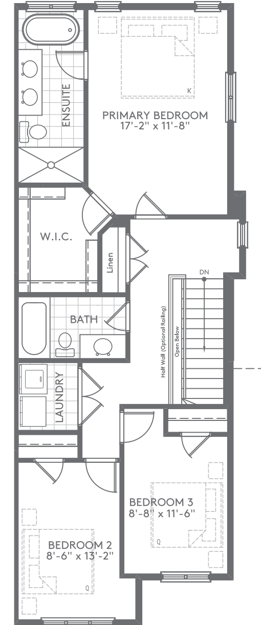
SECOND LEVEL
