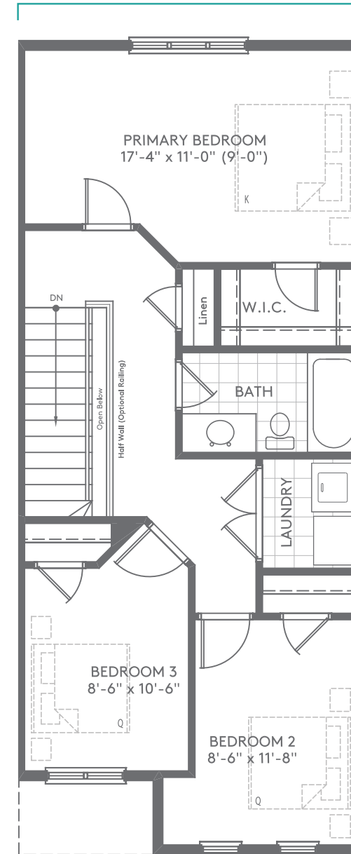
SECOND LEVEL
