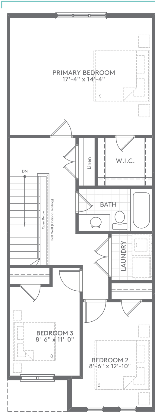
SECOND LEVEL
