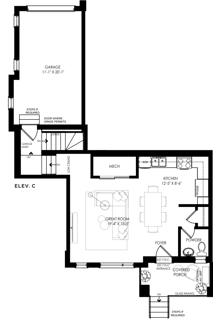
FIRST LEVEL FRONT
