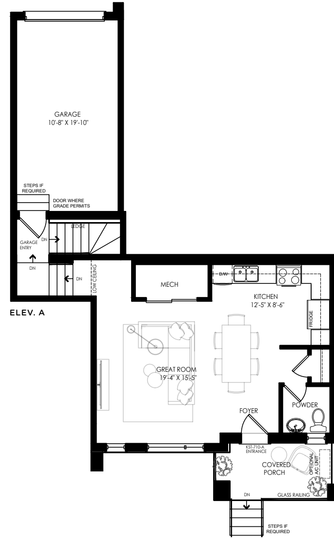
FIRST LEVEL FRONT
