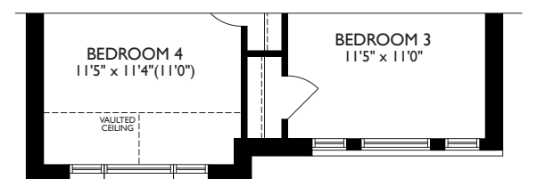
UPPER LEVEL - ELEV. C
