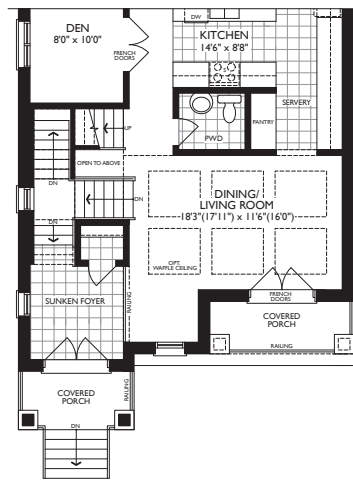
PART. MAIN LEVEL - ELEV. C
