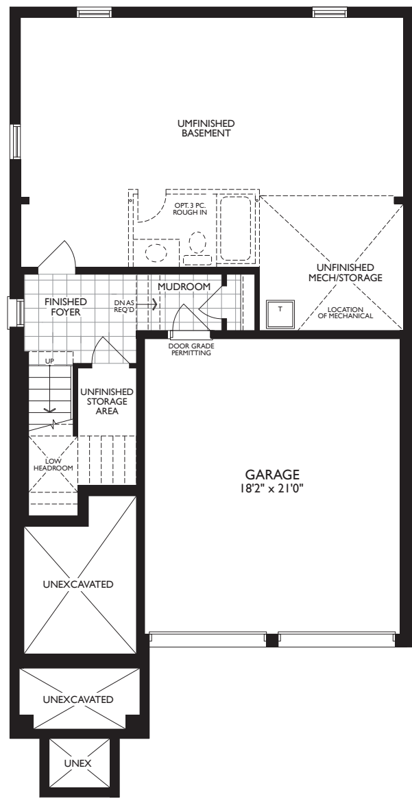
GROUND LEVEL - ELEV. A
