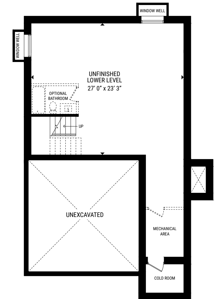
LOWER LEVEL
