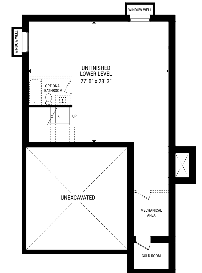
LOWER LEVEL
