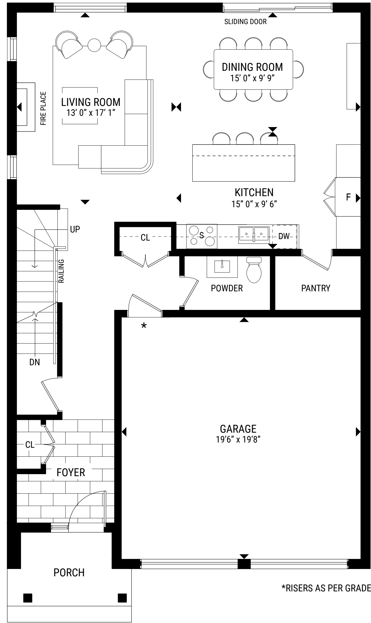
MAIN LEVEL
