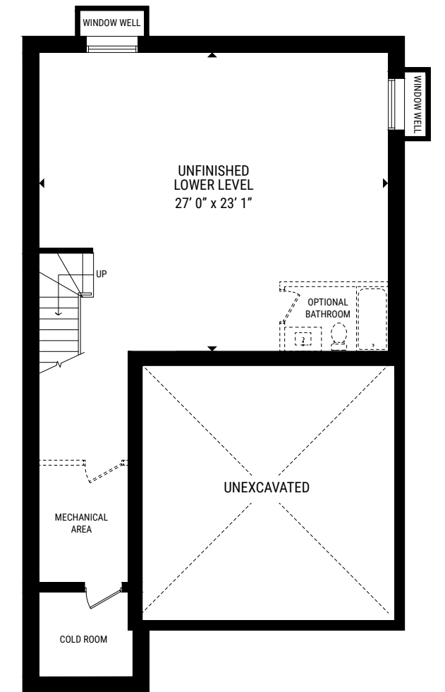
LOWER LEVEL
