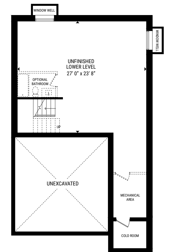
LOWER LEVEL
