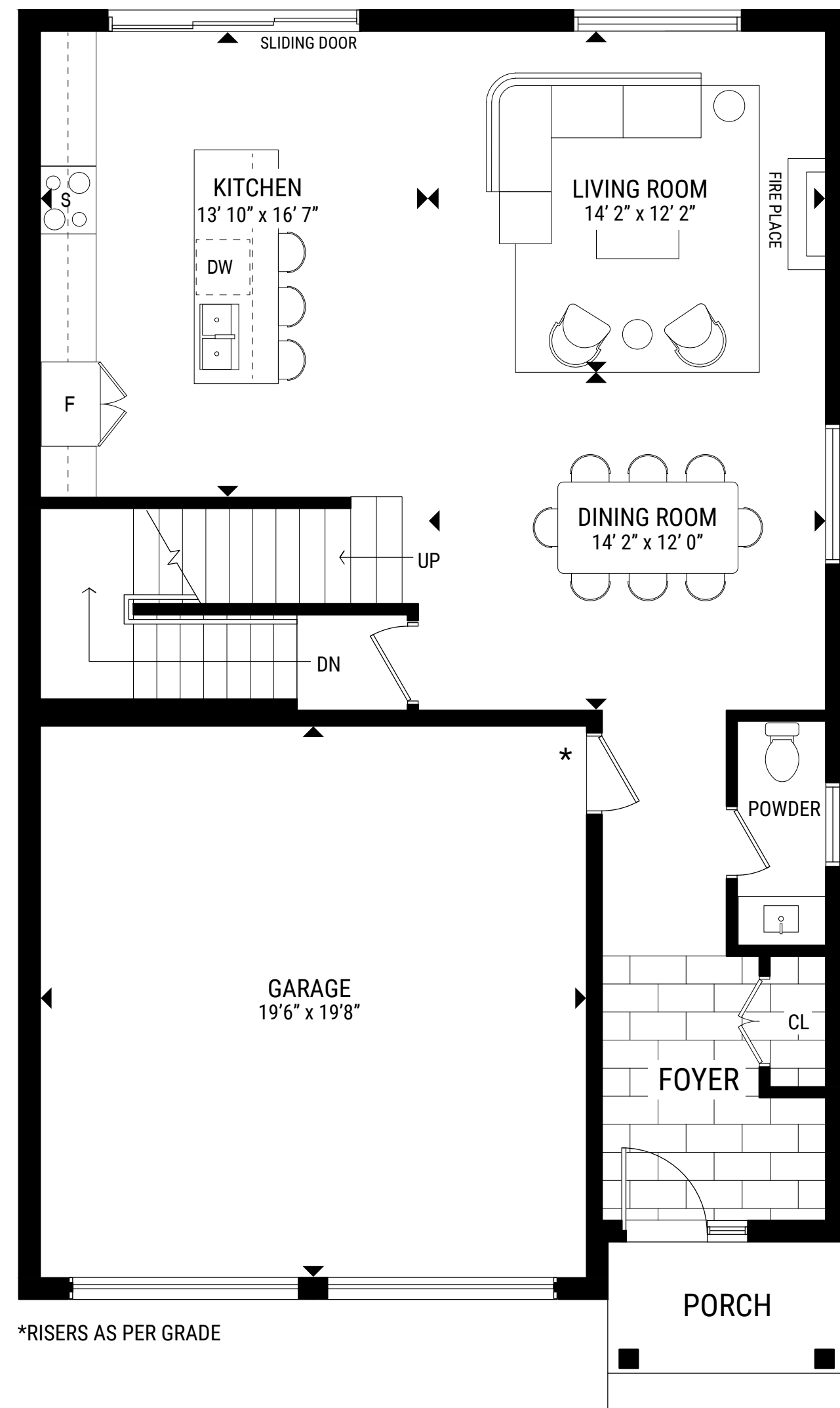
MAIN LEVEL
