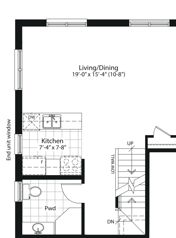
ELEV. A LEVEL 3
