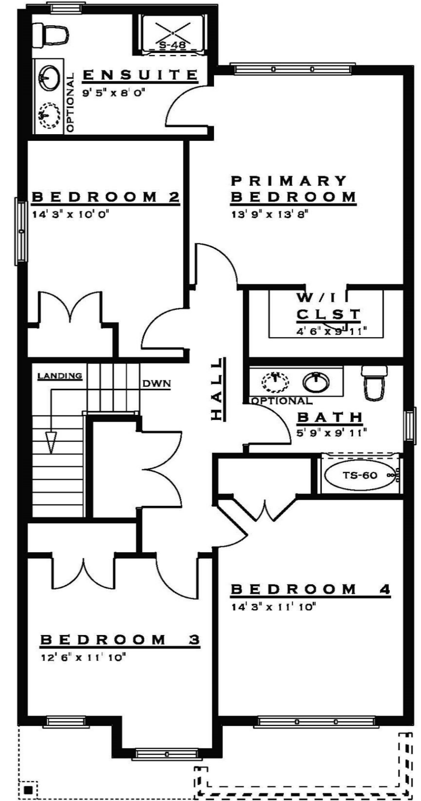
SECOND FLOOR
