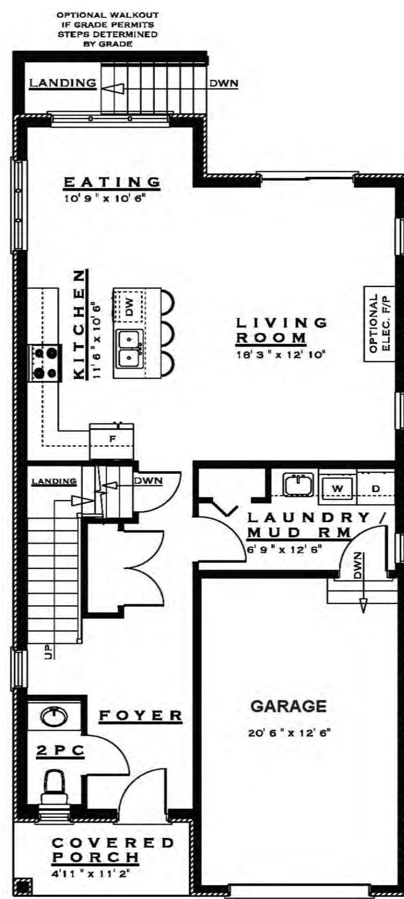
MAIN FLOOR
