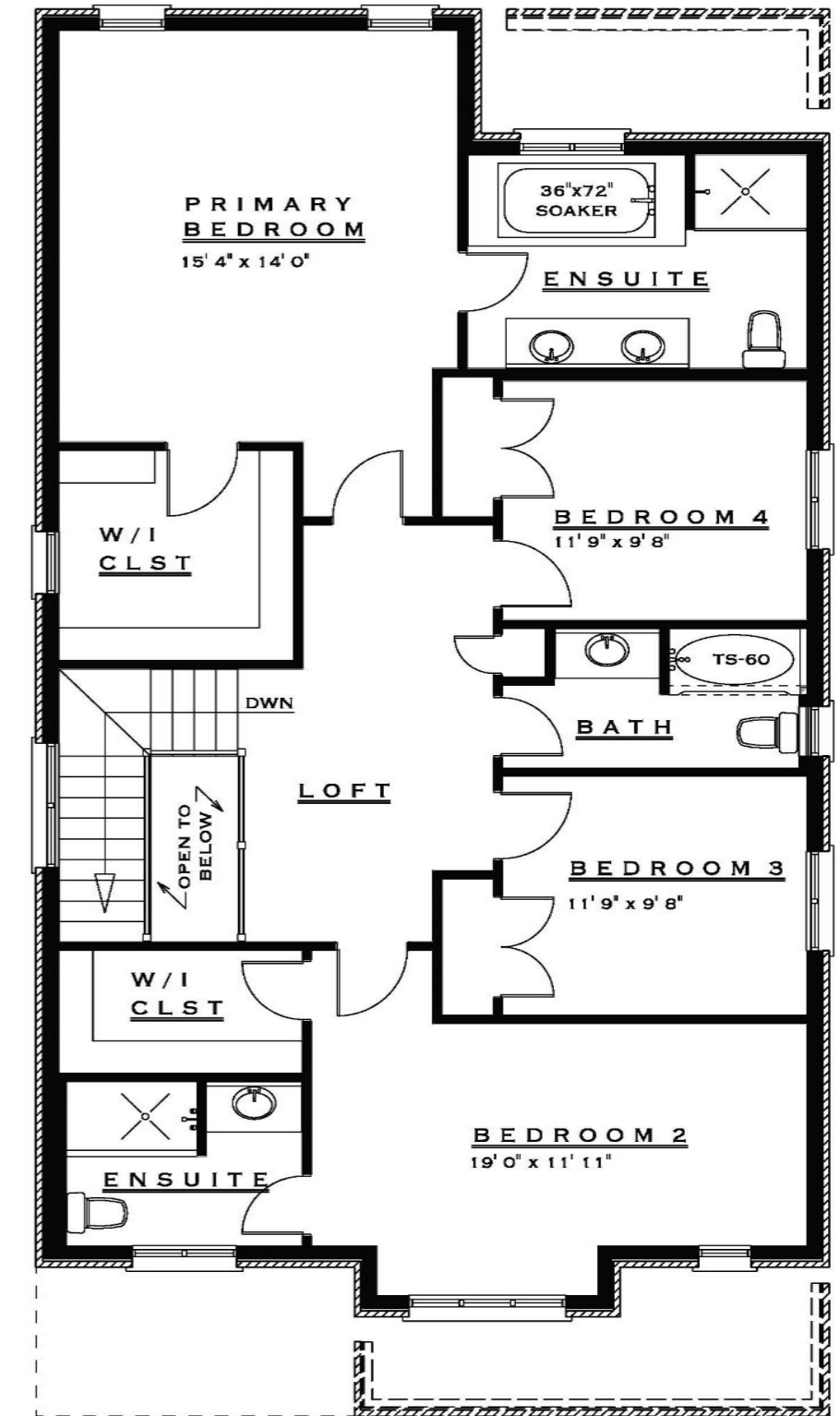
SECOND FLOOR
