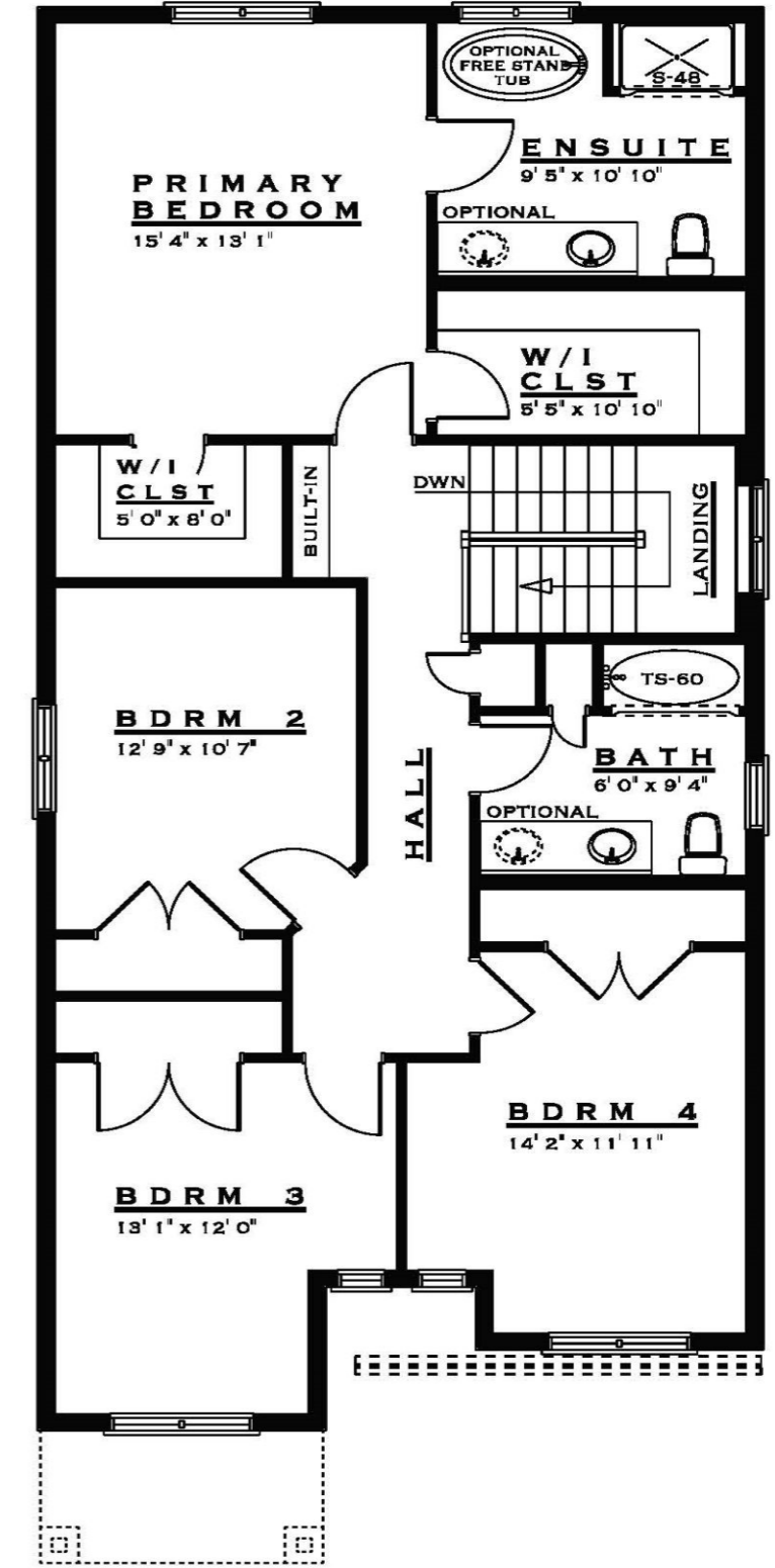
SECOND FLOOR
