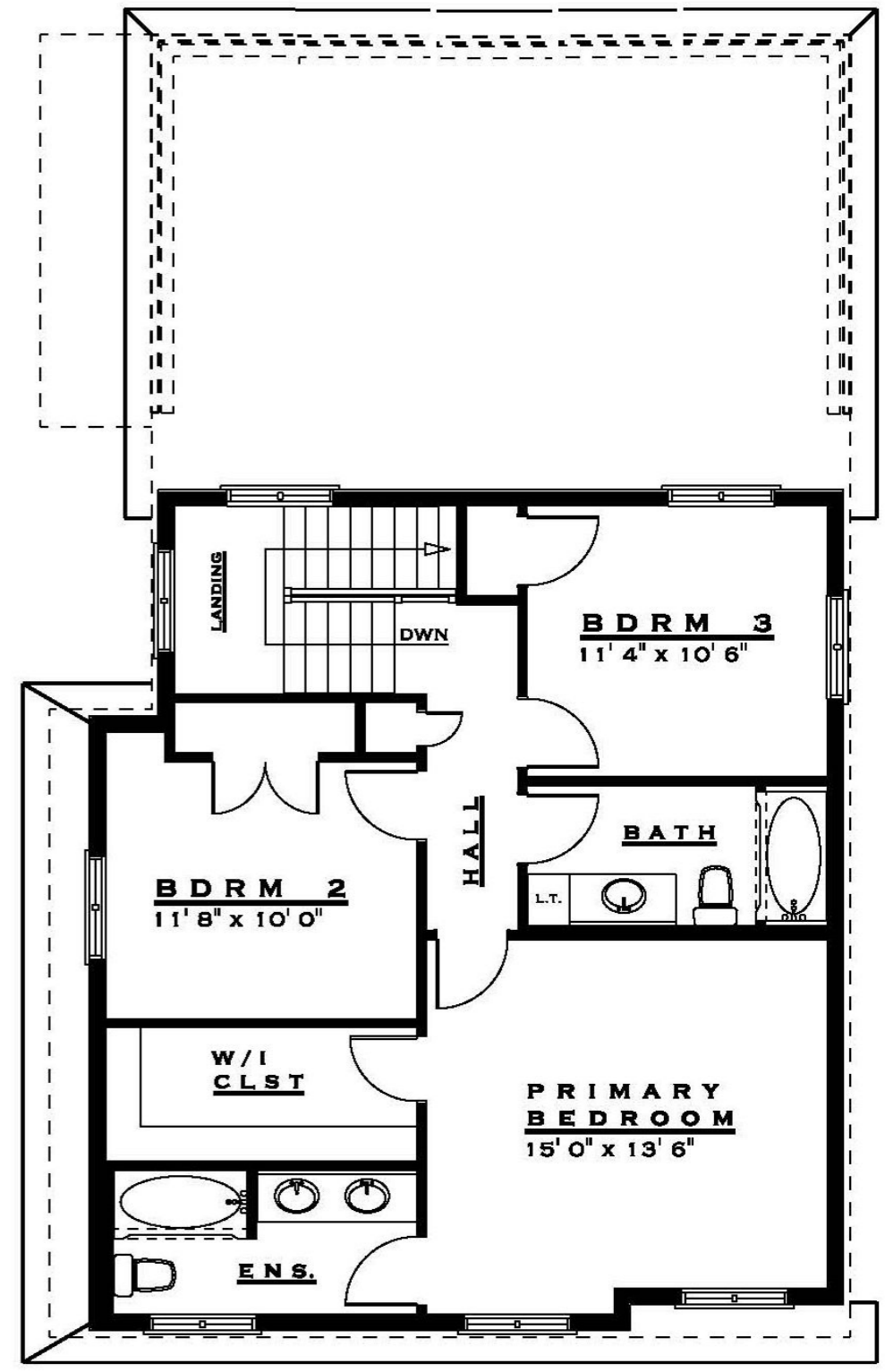
SECOND FLOOR
