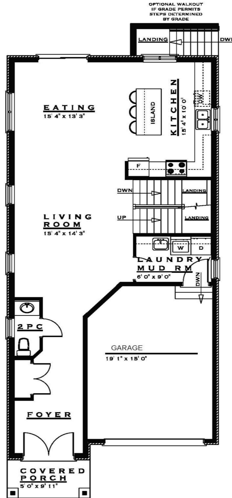
MAIN FLOOR
