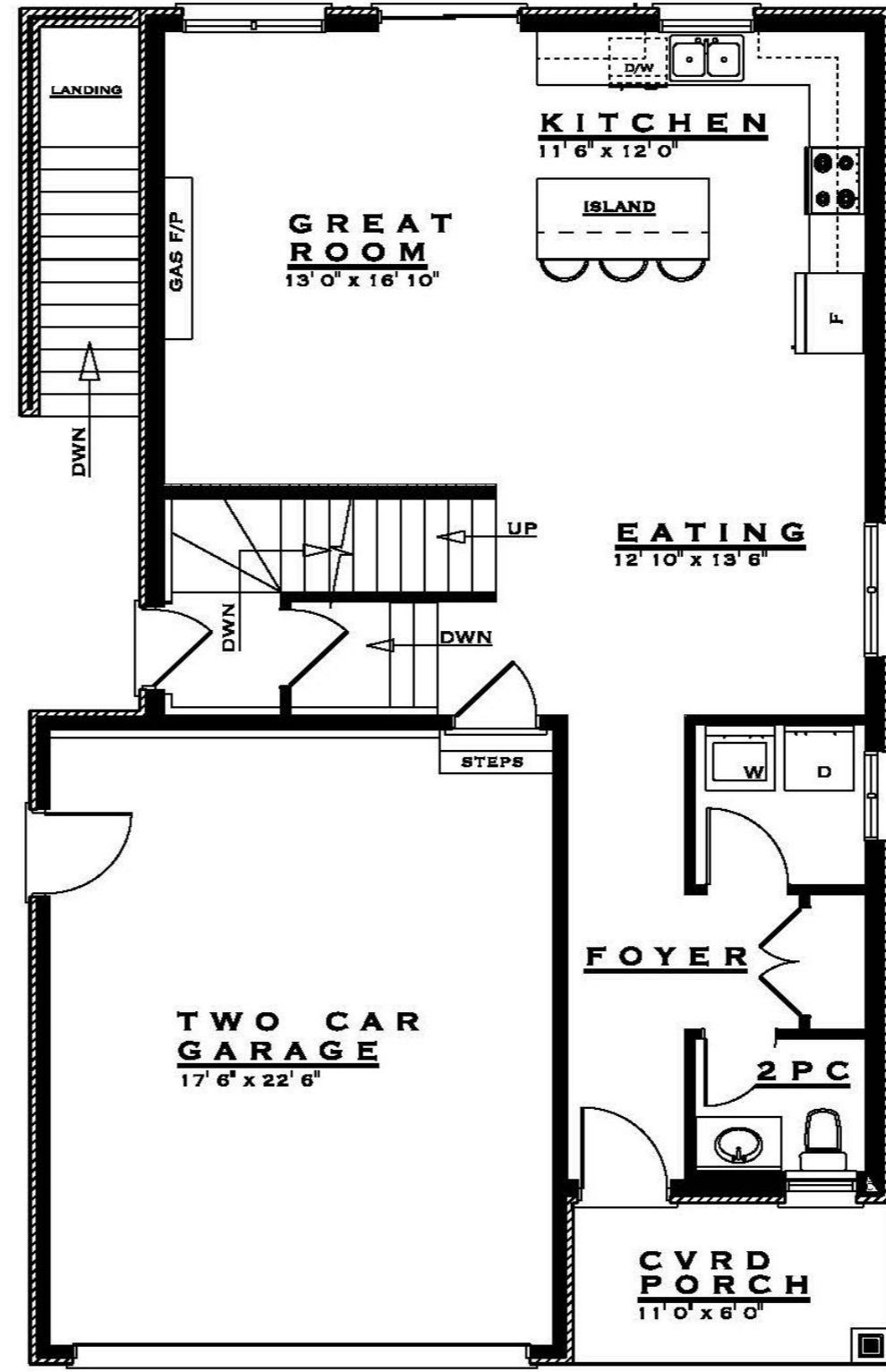
MAIN FLOOR
