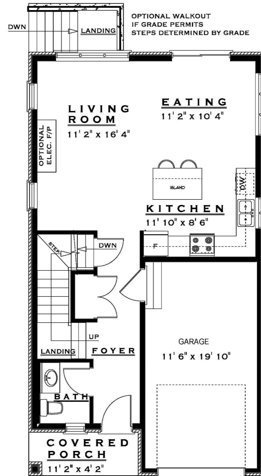
MAIN FLOOR
