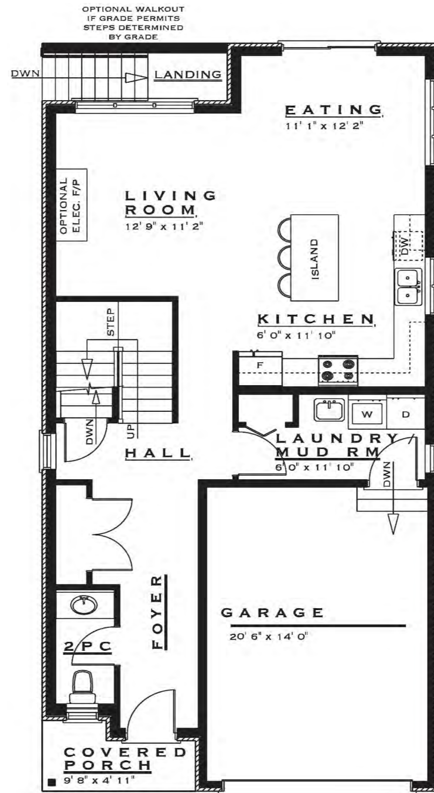
MAIN FLOOR
