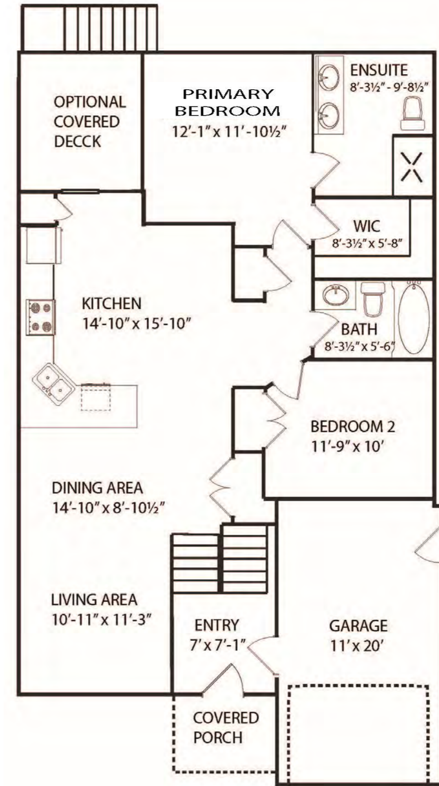
MAIN FLOOR
