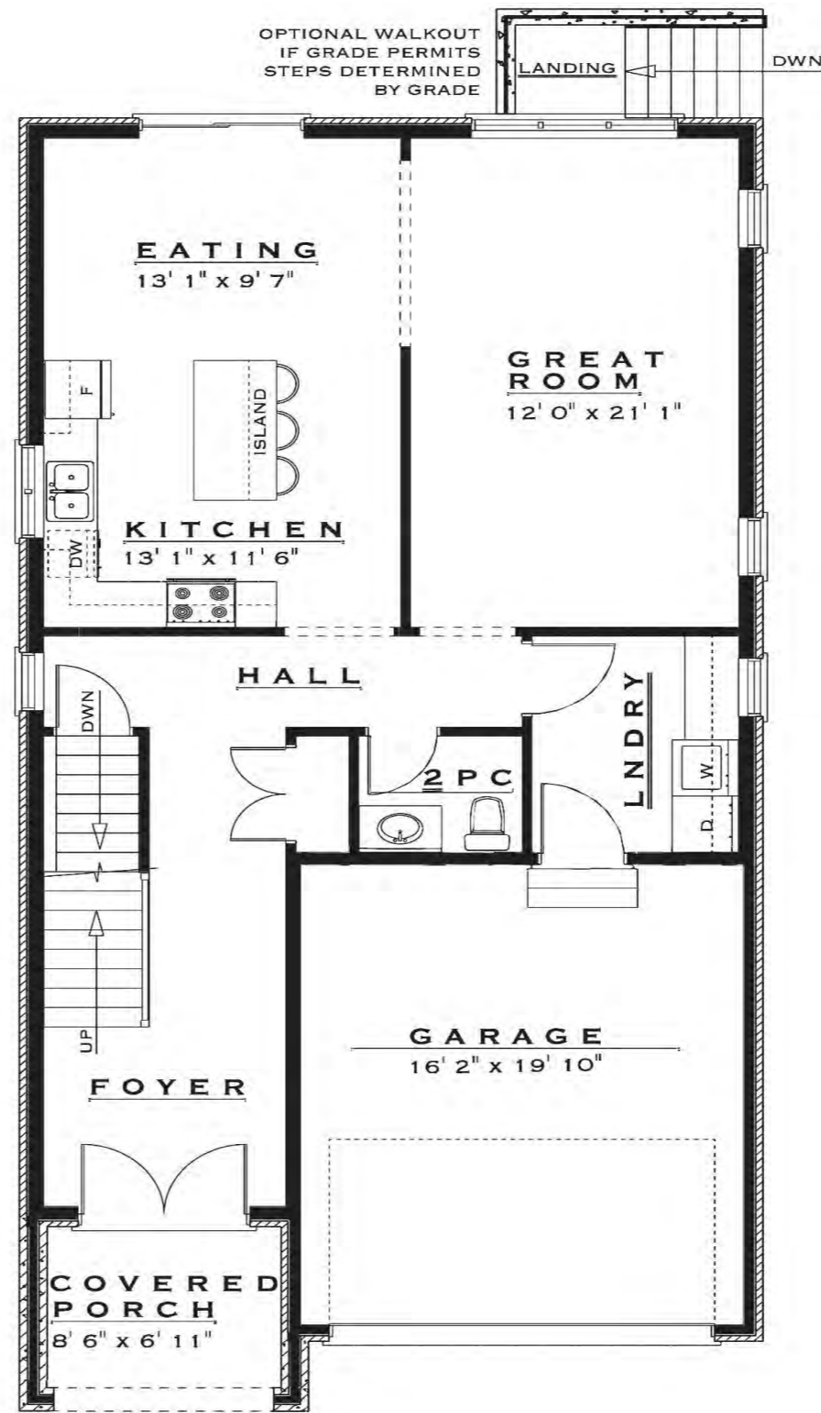
MAIN FLOOR
