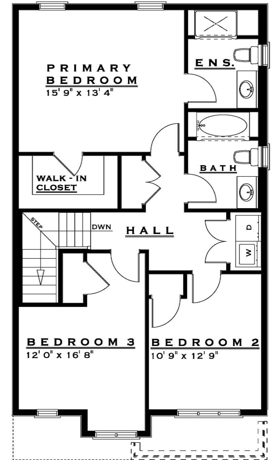
SECOND FLOOR
