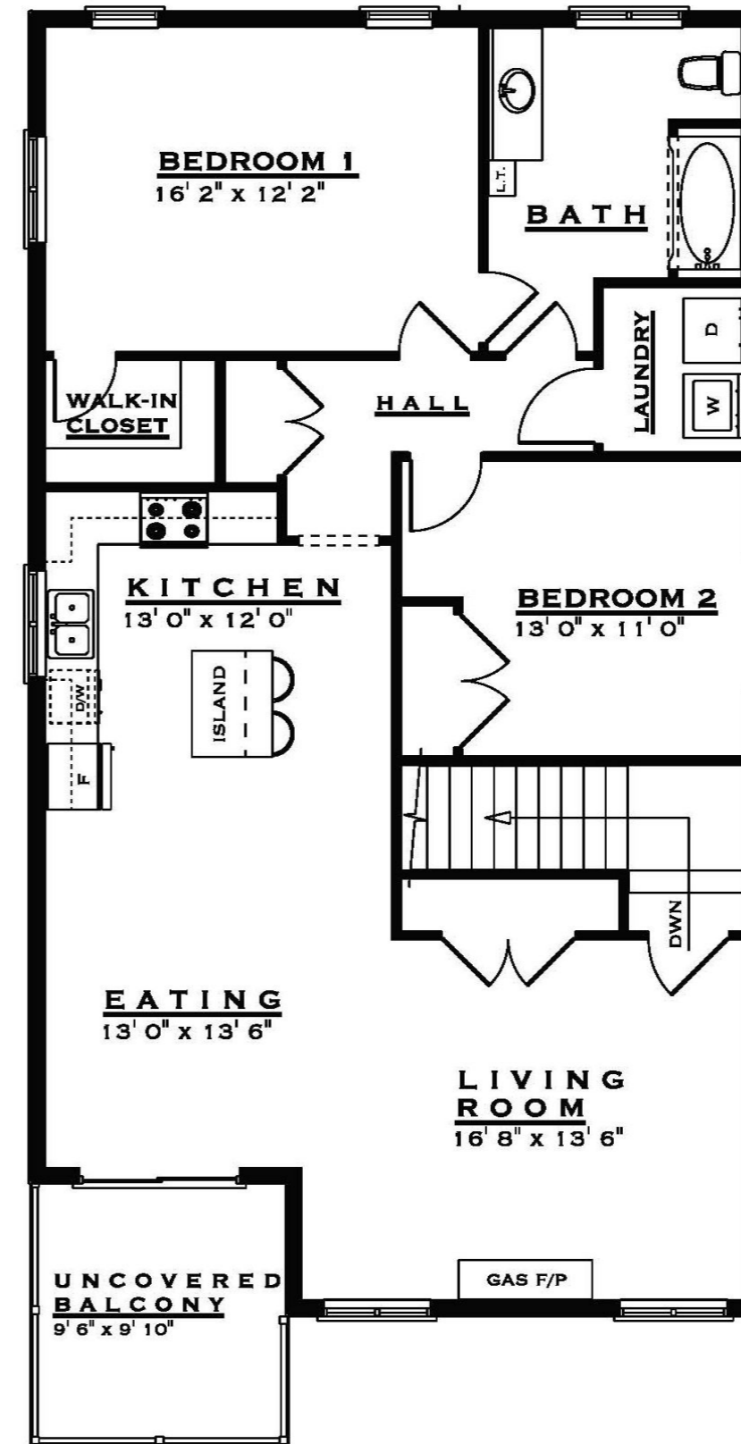
SECOND FLOOR
