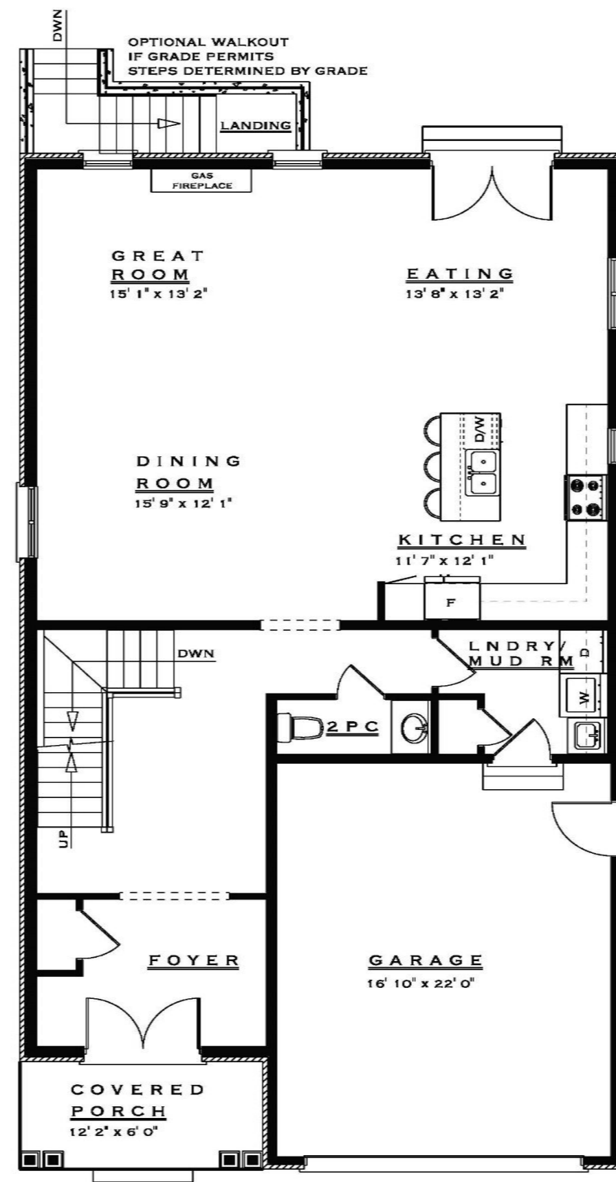
MAIN FLOOR
