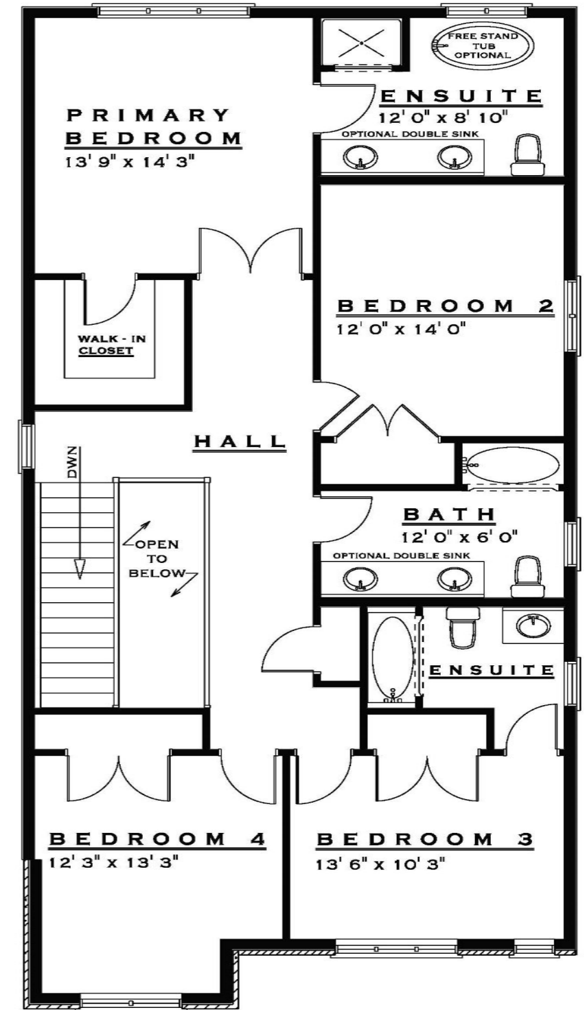
SECOND FLOOR
