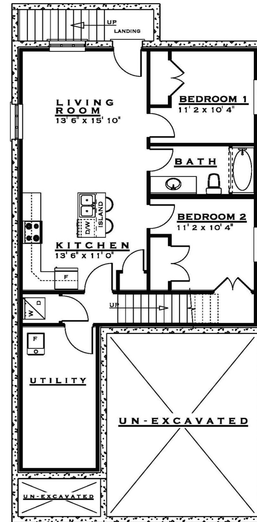
OPTIONAL FINISHED BASEMENT
