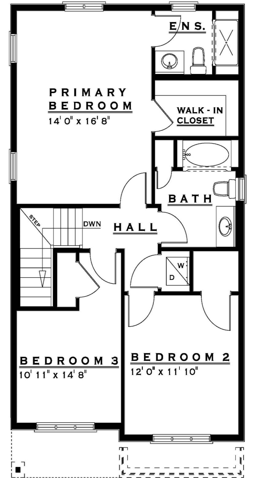
SECOND FLOOR
