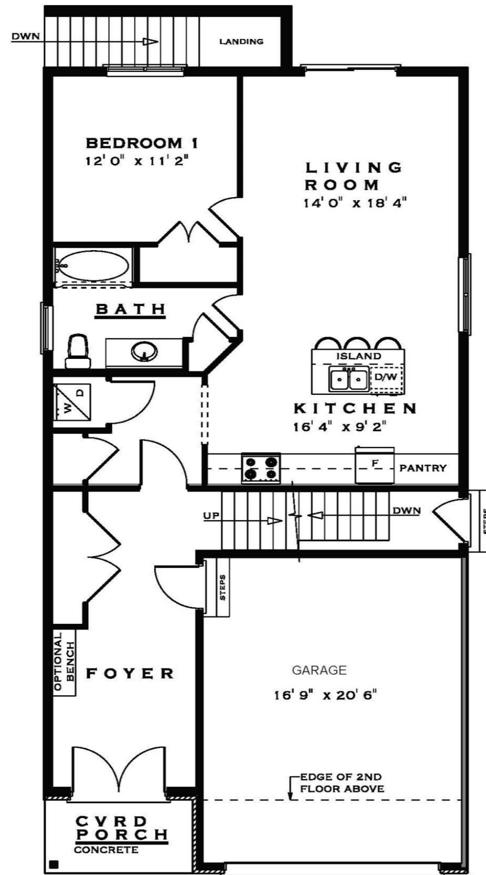
MAIN FLOOR
