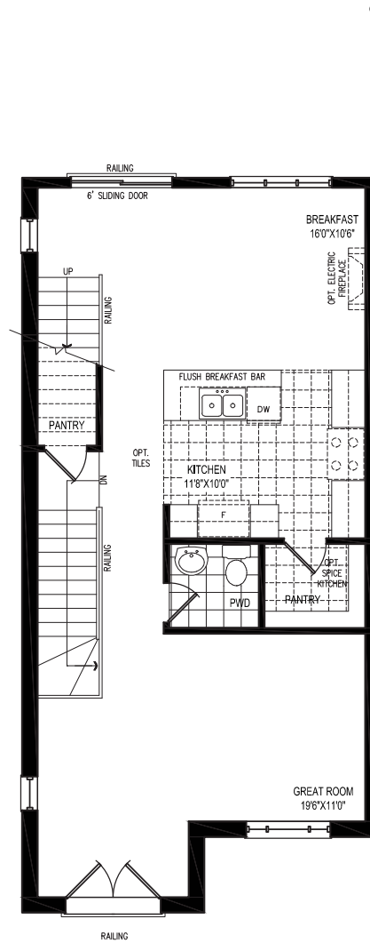
Living Level Plan
