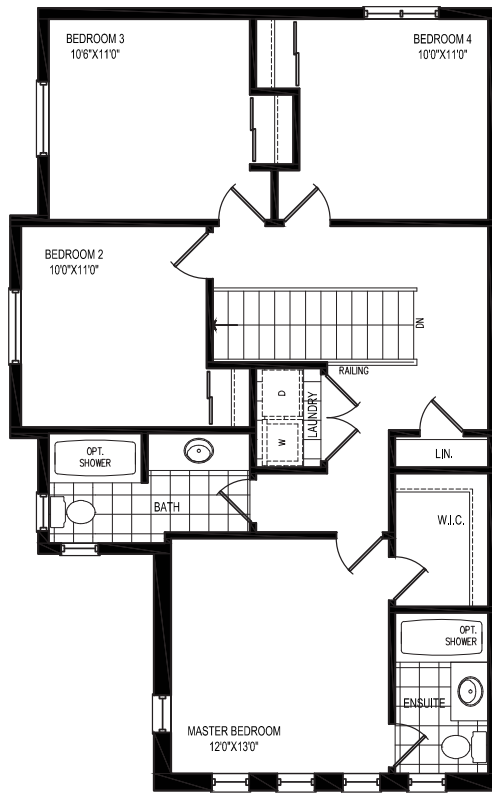
Sleeping Level Plan "B"
