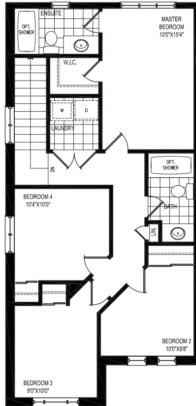
Alt. Sleeping Level Plan - 4 Bed
