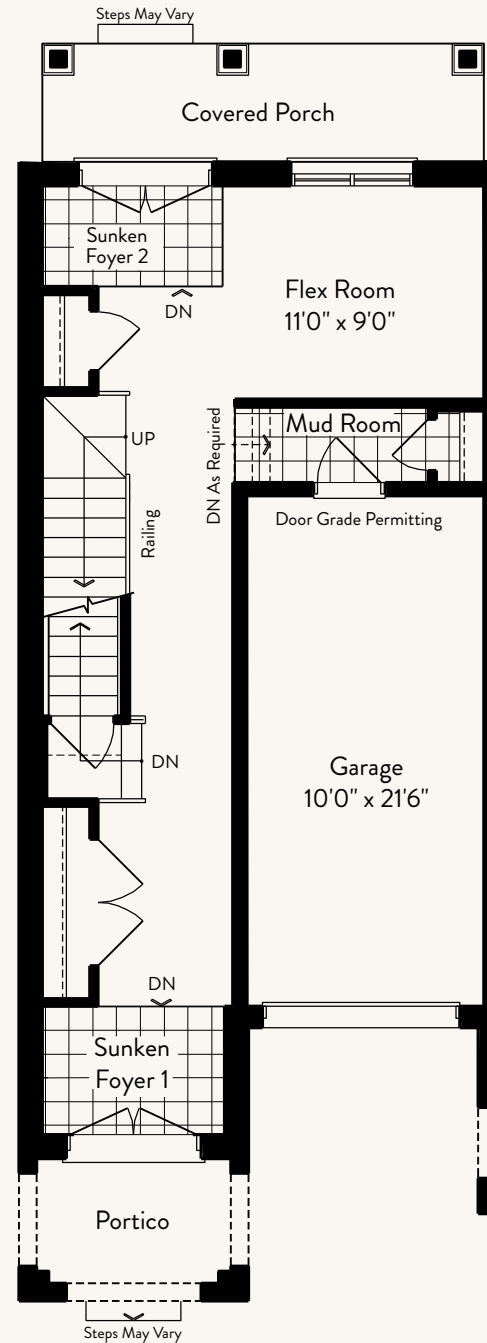
Ground Floor
