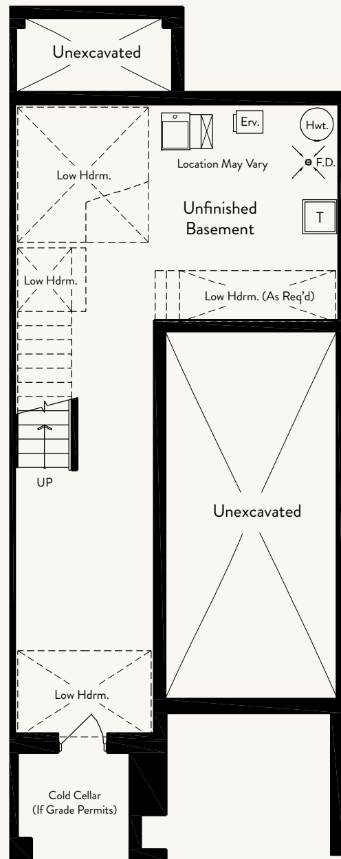
Basement
