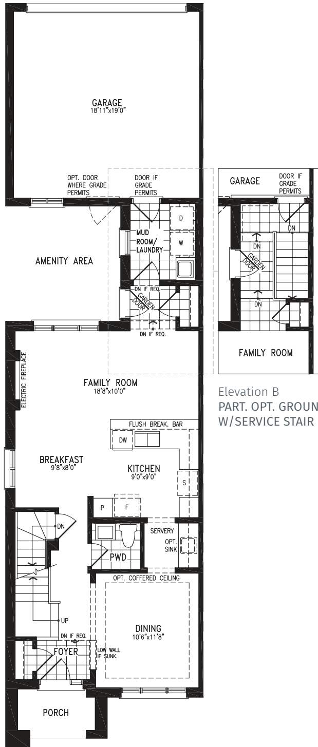
Elevation B GROUND FLOOR
