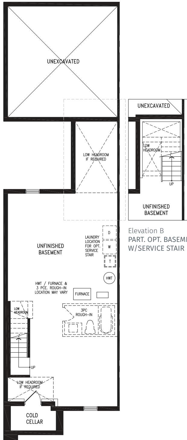
Elevation B BASEMENT
