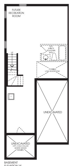
BASEMENT ELEVATION 'A'
