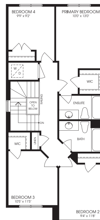
OPTIONAL SECOND FLOOR W/ 4 BEDROOMS ELEVATION 'A'
