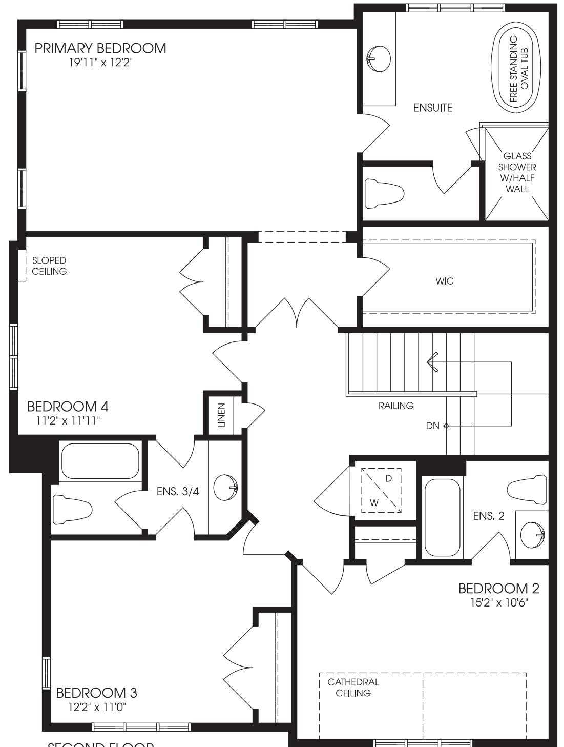
SECOND FLOOR ELEVATION 'A'
