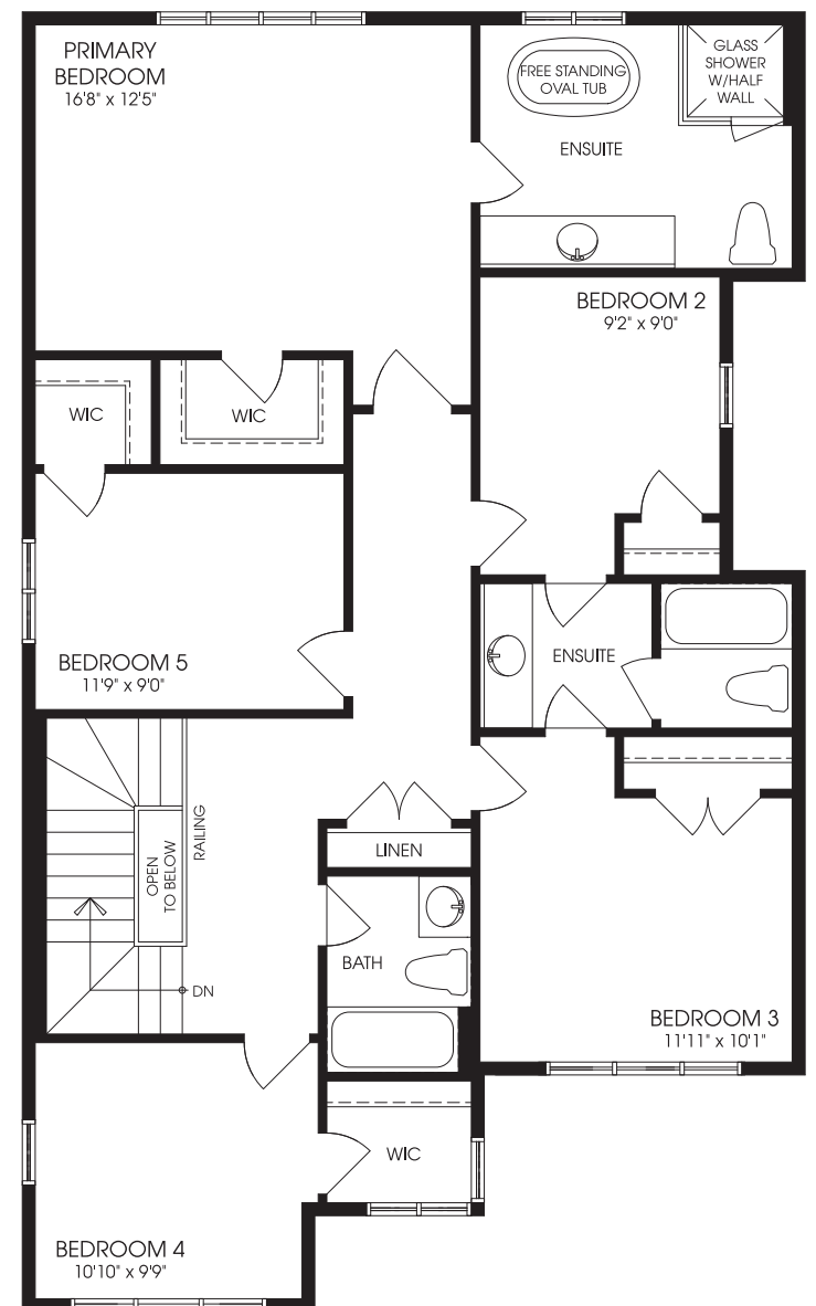
OPT. 5 BEDROOM SECOND FLOOR ELEVATION 'A'
