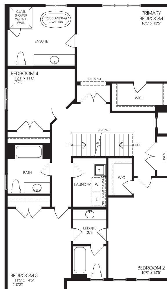
SECOND FLOOR W/ LOFT ELEVATION 'A'
