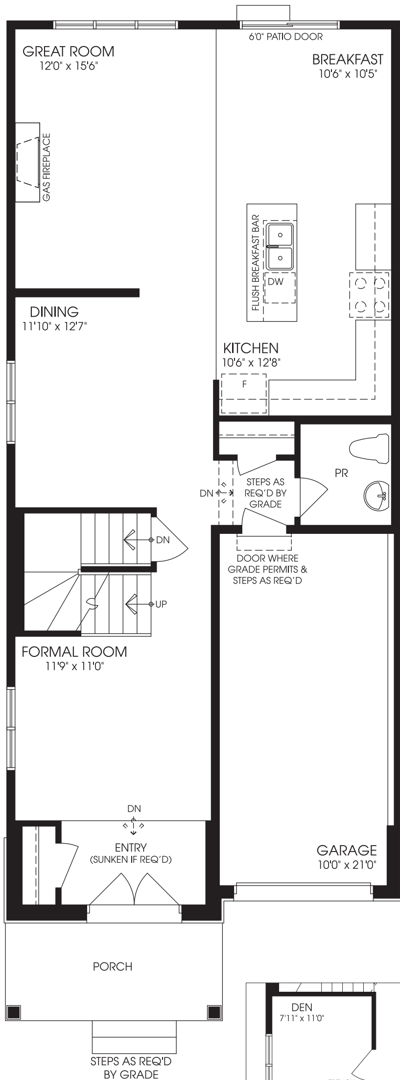
MAIN FLOOR ELEVATION 'A'
