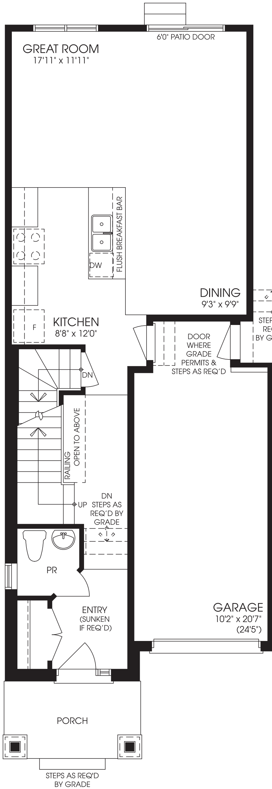
MAIN FLOOR ELEVATION 'A1'
