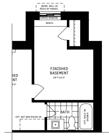
8 Finished Basement Package
