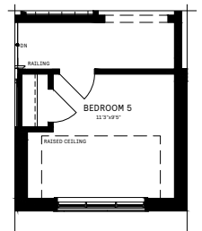
8 5 Bedroom Plan
