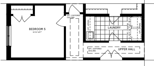
5 2nd Floor 5 Bedroom Plan
