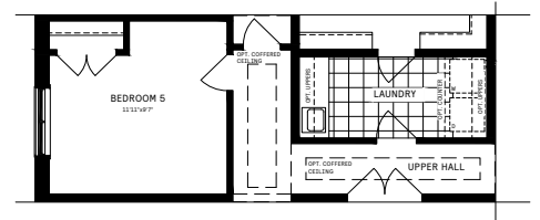
8 5 Bedroom Plan
