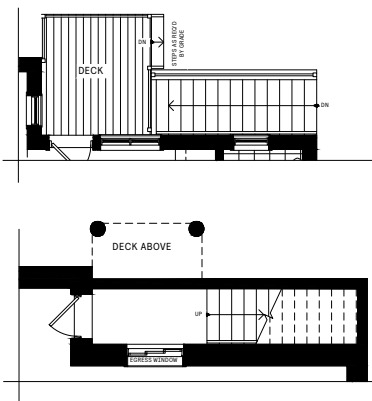
2 Walk-Up Steps
