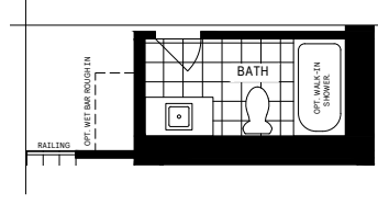
7 Finished Basement Bathroom
