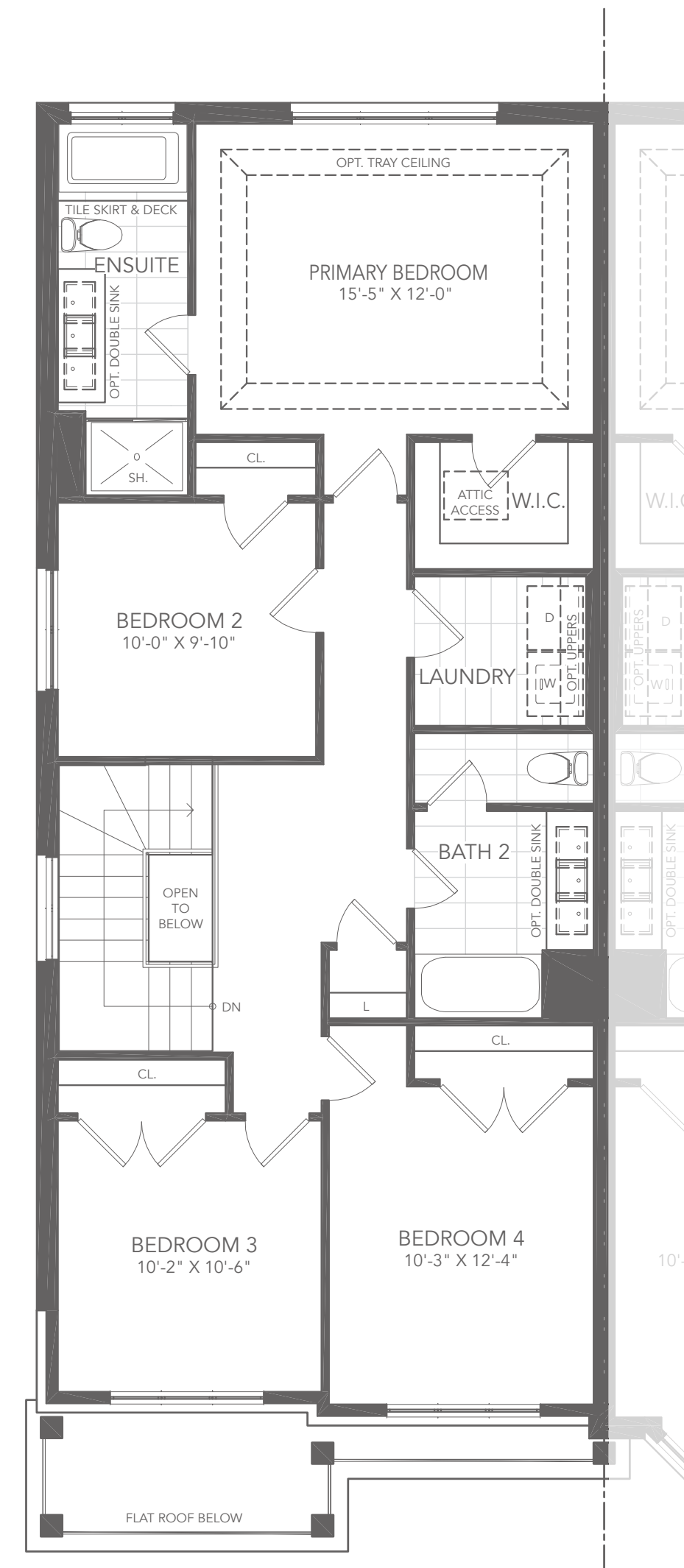
SECOND FLOOR PLAN A
