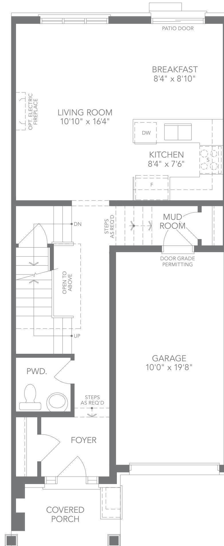
U2 ELEV. A1 GROUND FLOOR PLAN
