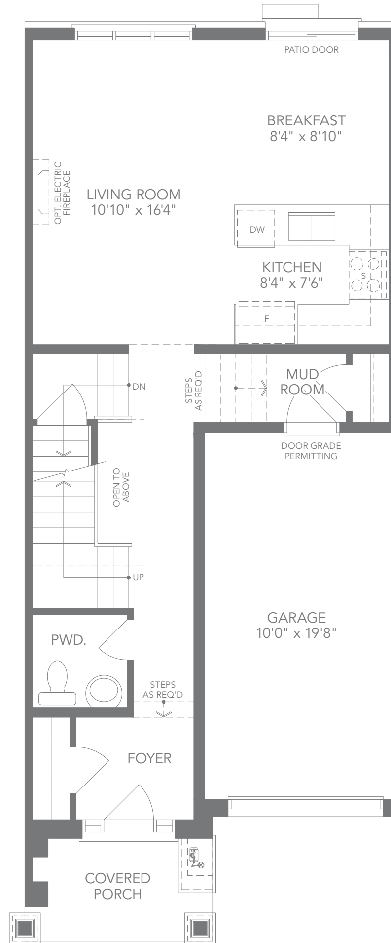
U2 ELEV. C2 GROUND FLOOR PLAN
