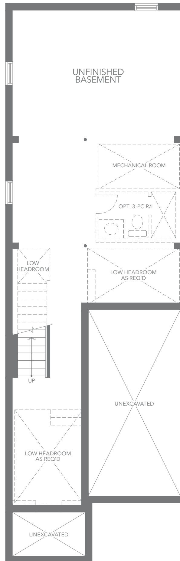
T3 END - ELEV. A3 BASEMENT FLOOR PLAN
