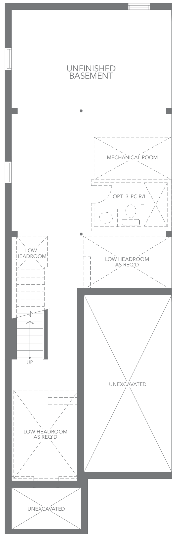
T3 END - ELEV. A3 MOD BASEMENT FLOOR PLAN
