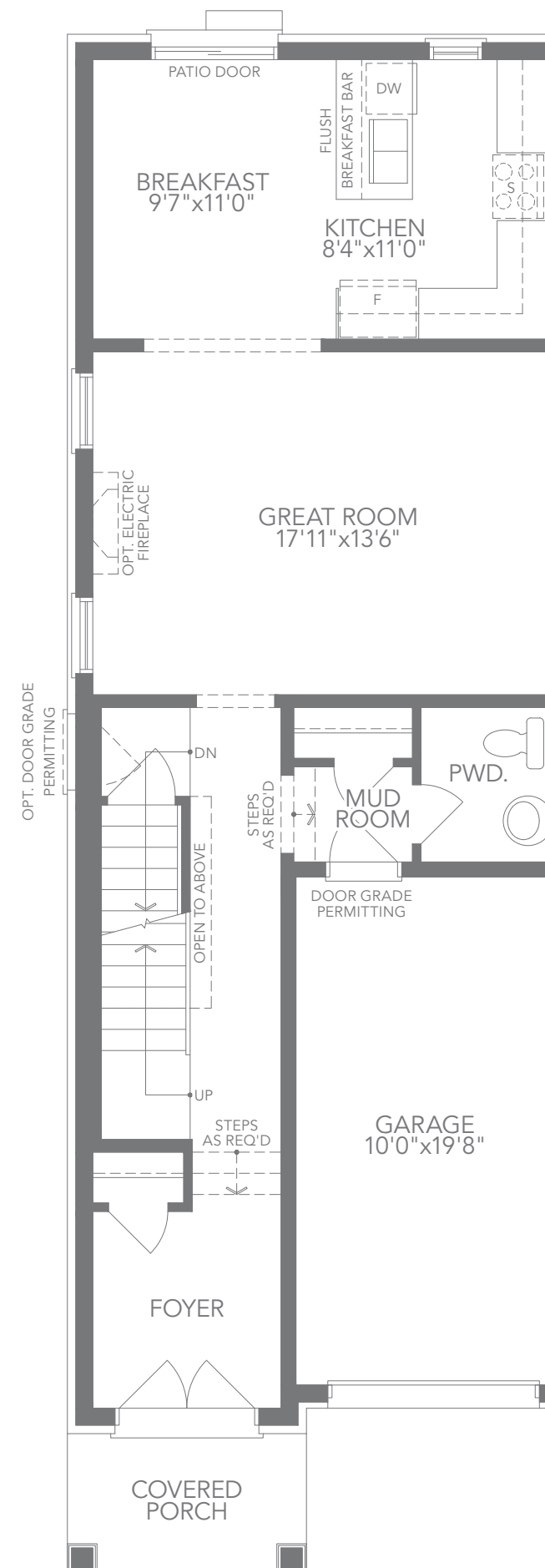
T3 END - ELEV. A3 GROUND FLOOR PLAN
