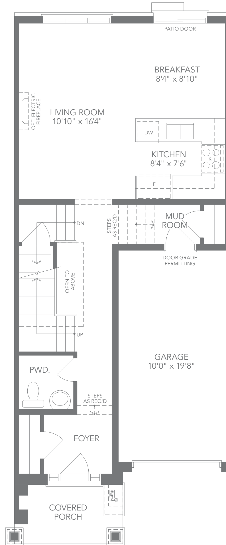
U2 ELEV. B2 GROUND FLOOR PLAN
