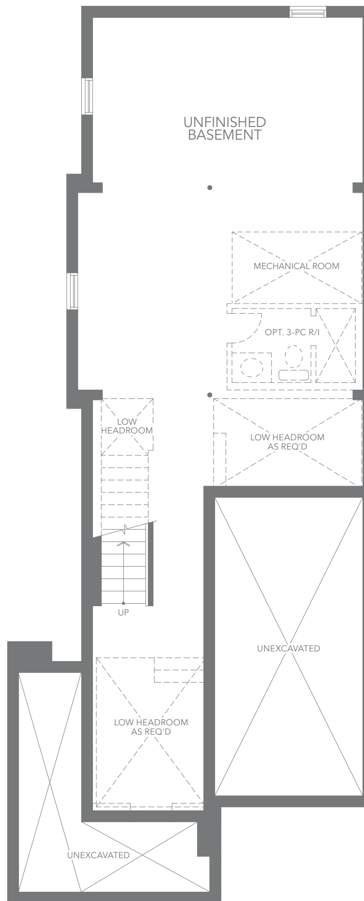
T3 COR - ELEV. A4 MOD BASEMENT FLOOR PLAN
