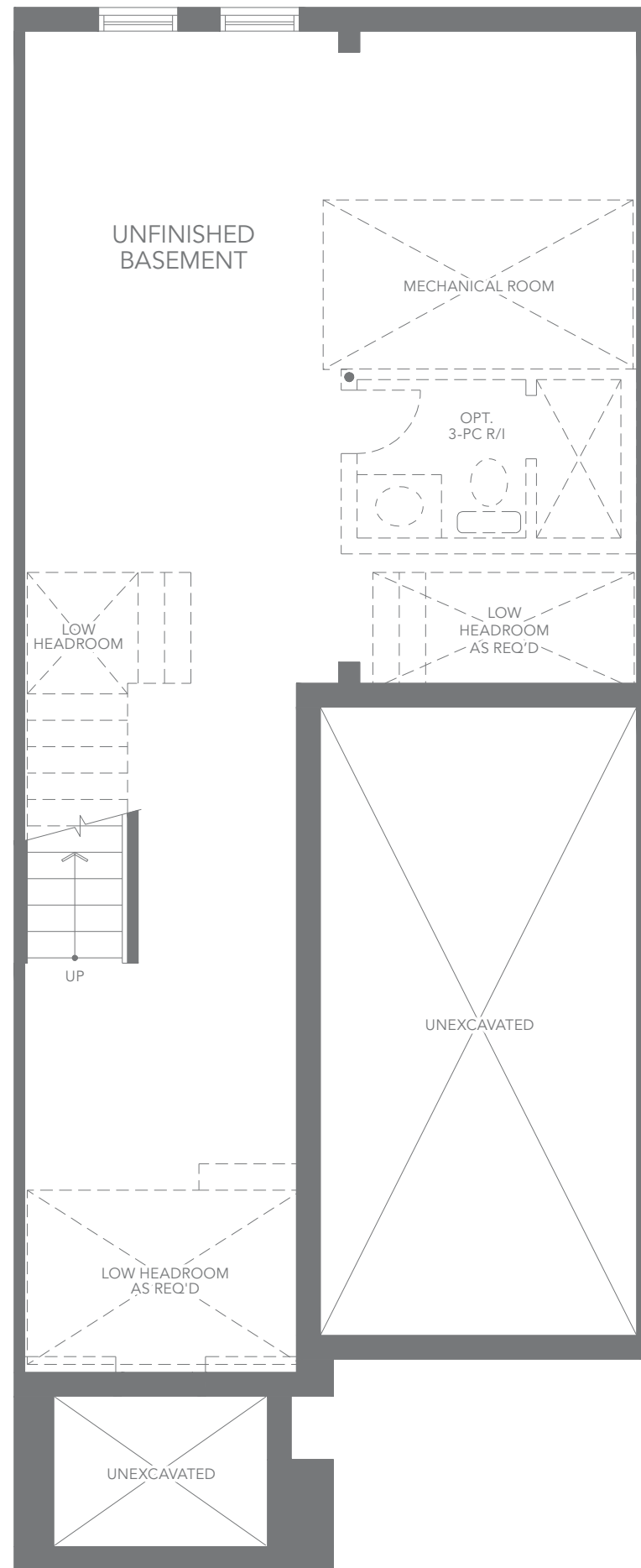
U2 ELEV. C1 BASEMENT FLOOR PLAN
