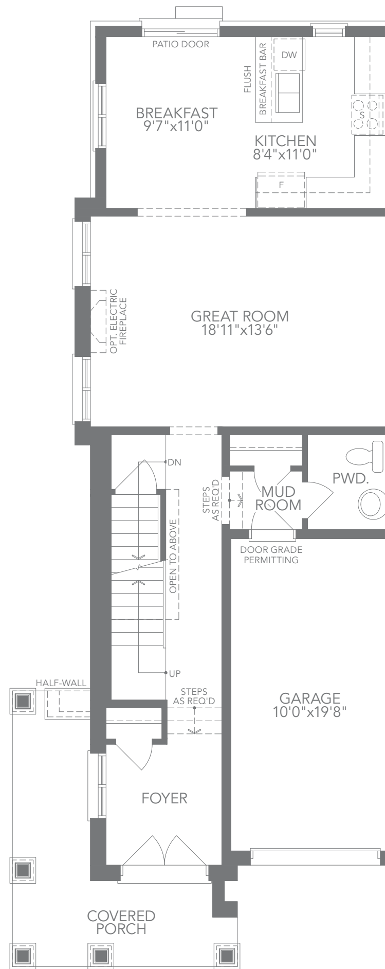
T3 COR - ELEV. C4 GROUND FLOOR PLAN
