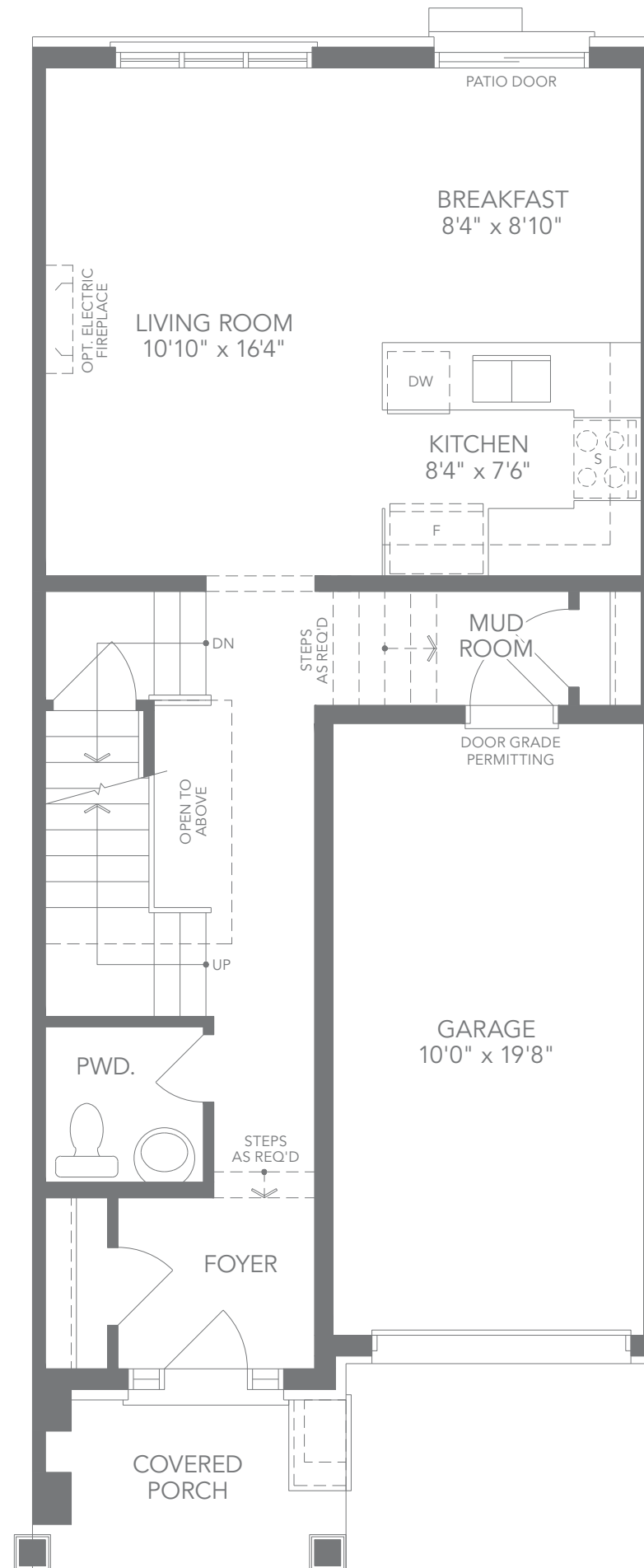
U2 ELEV. A2 GROUND FLOOR PLAN
