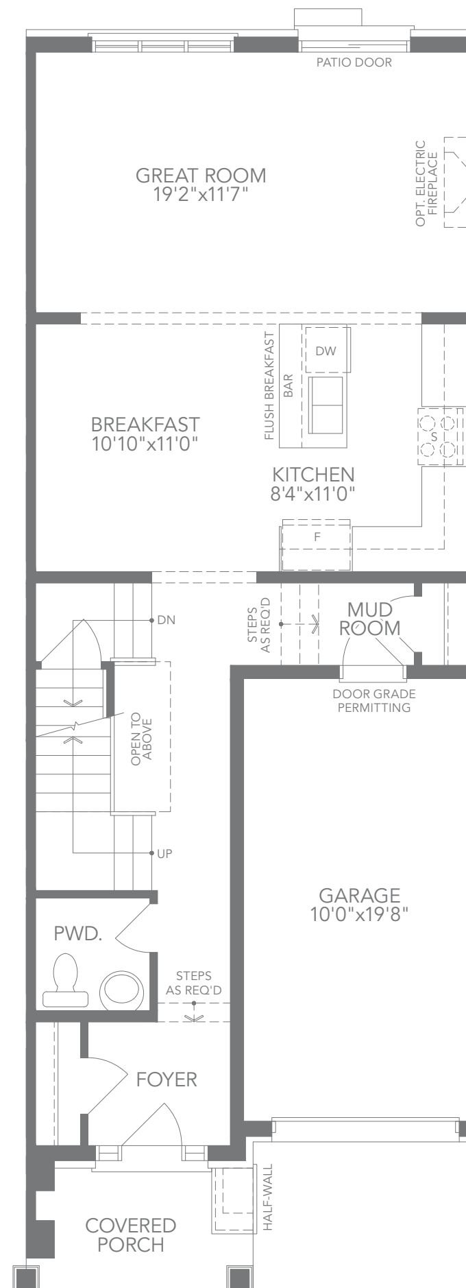
T1 - ELEV. A2 GROUND FLOOR PLAN
