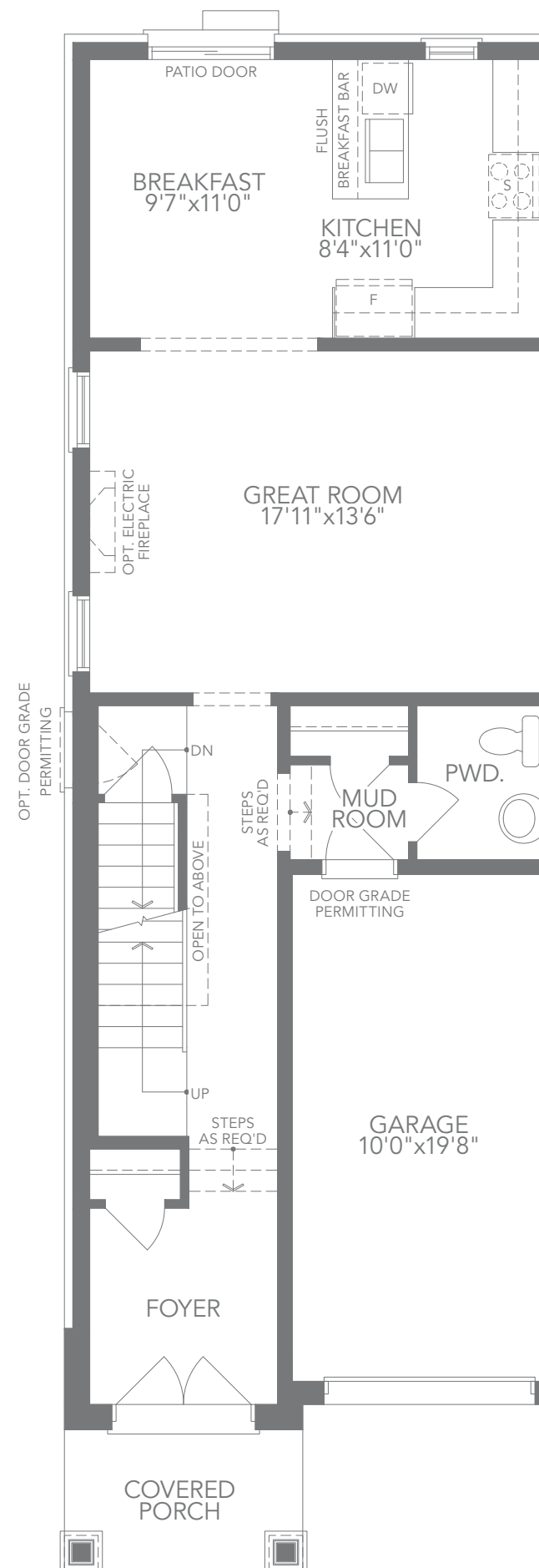
T3 END - ELEV. C3 MOD GROUND FLOOR PLAN
