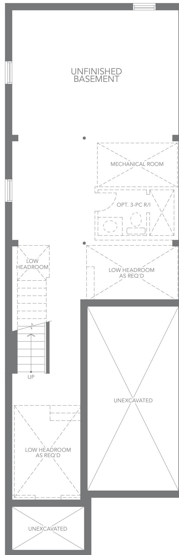
T3 END - ELEV. B3 BASEMENT FLOOR PLAN
