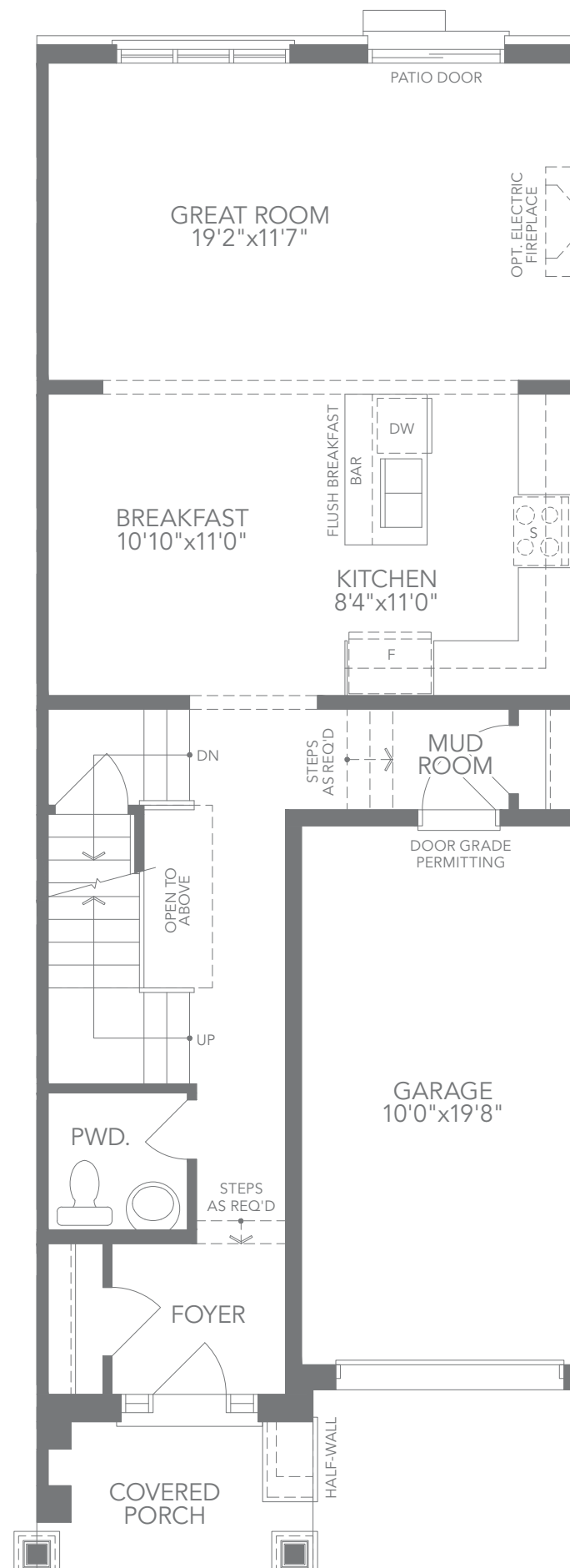
T1 - ELEV. B1 GROUND FLOOR PLAN
