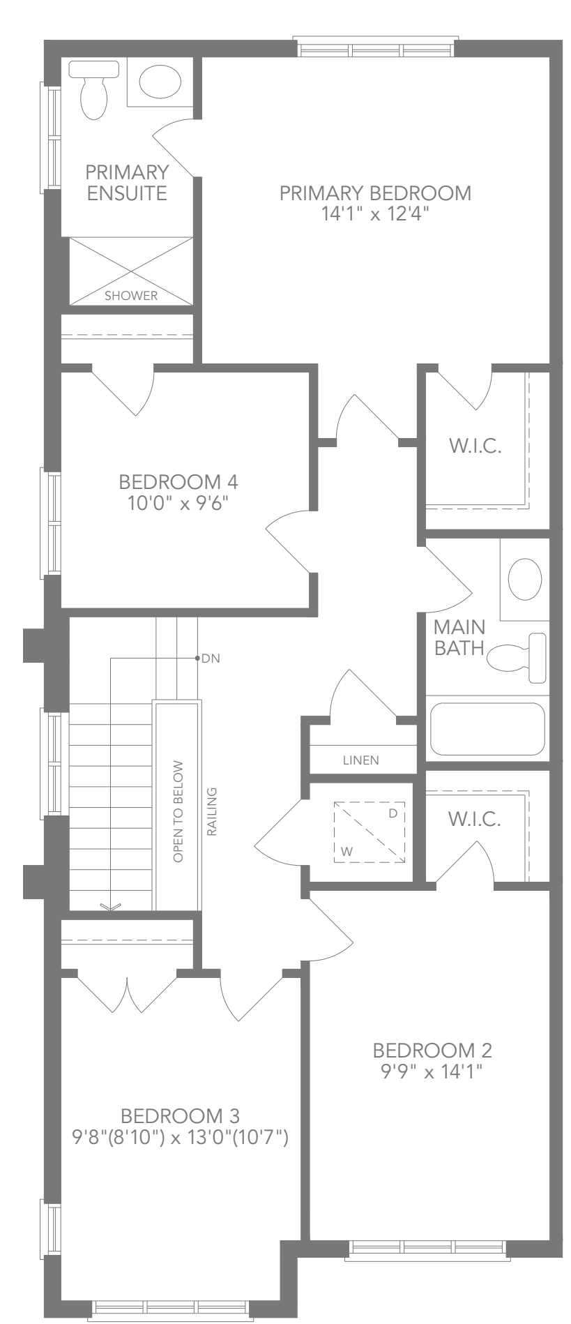
ELEV. A3 OPT. UPPER FLOOR PLAN
