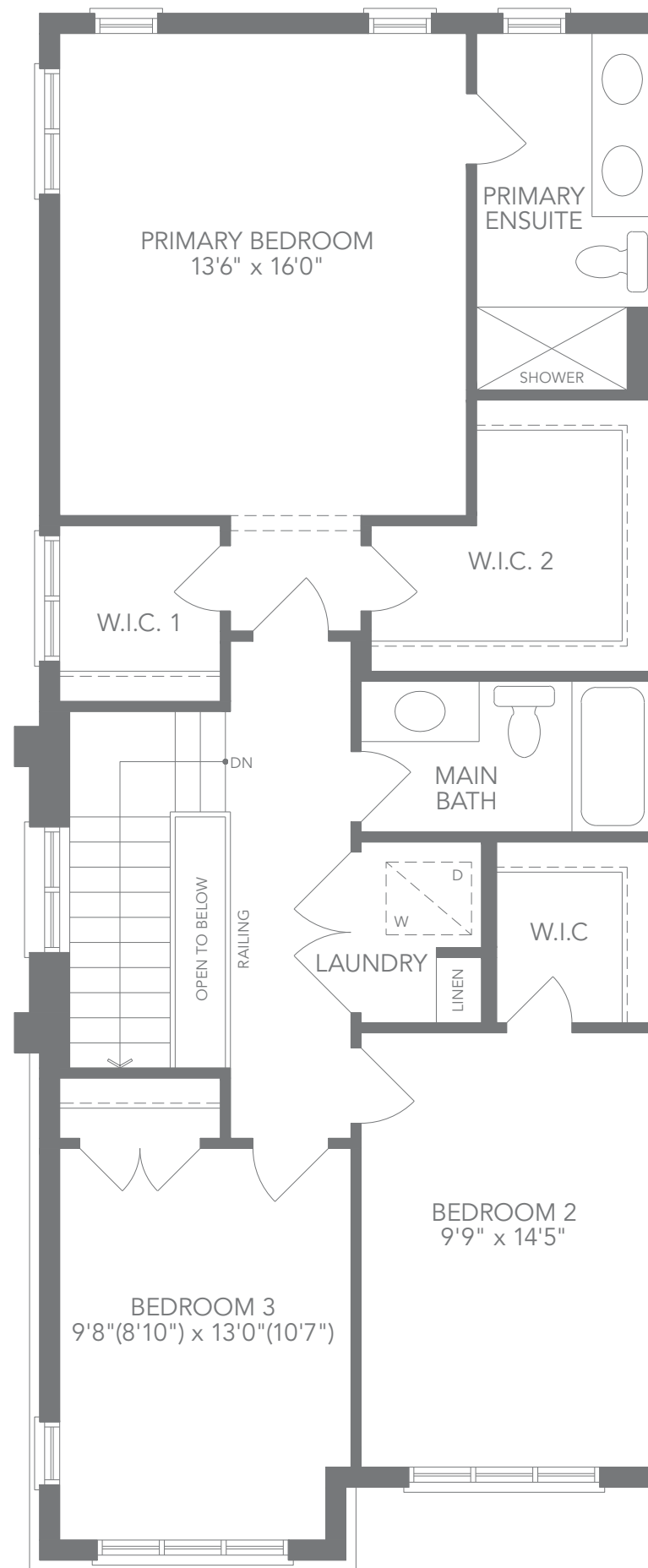
ELEV. C3 UPPER FLOOR PLAN
