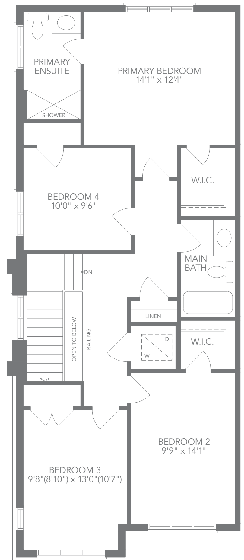
ELEV. C3 OPT. UPPER FLOOR PLAN
