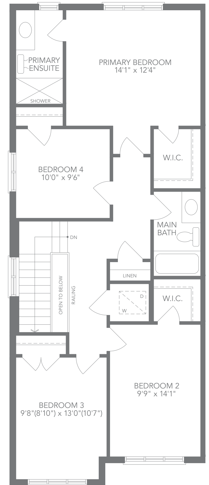
ELEV. A1 OPT. UPPER FLOOR PLAN
