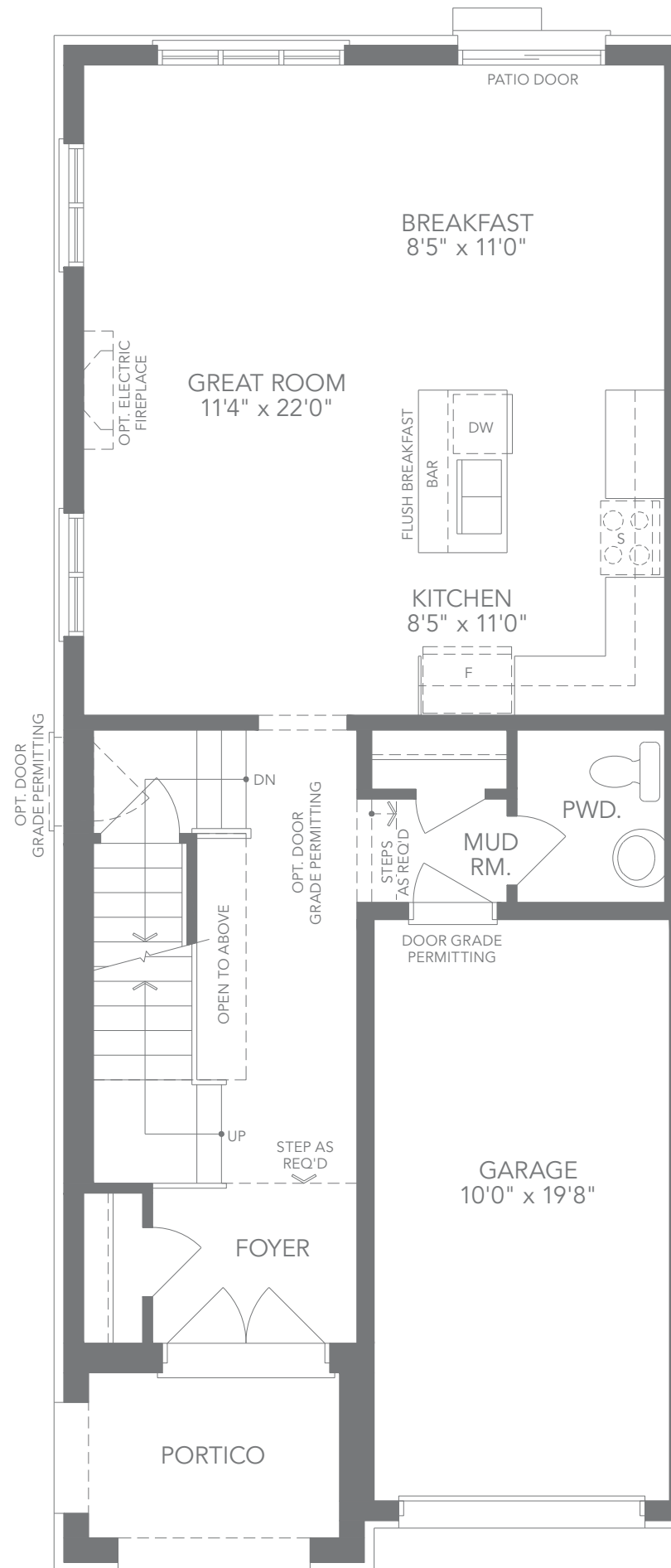
ELEV. A1 GROUND FLOOR PLAN
