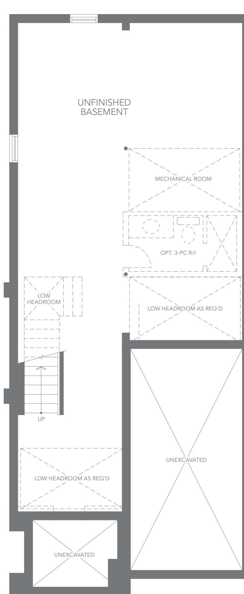
ELEV. B3 BASEMENT FLOOR PLAN
