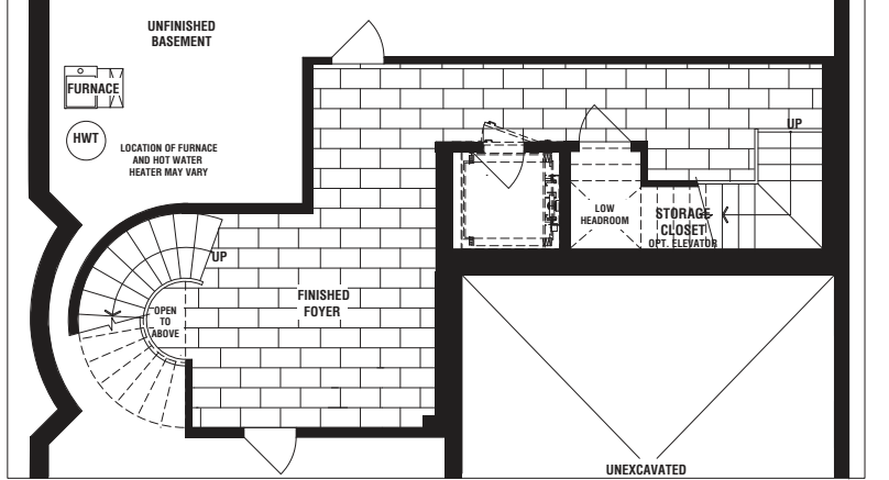
PARTIAL BASEMENT PLAN W/ SERVICE STAIR FOR OPT. ELEVATOR AND STORAGE
