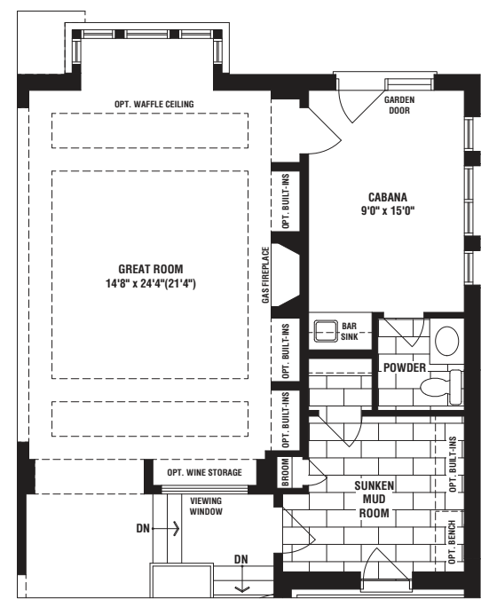
PARTIAL OPT. GROUND FLOOR PLAN W/ CABANA
