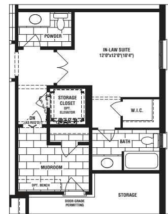
PARTIAL OPT. IN-LAW SUITE ELEV. 'A' (ELEV. 'B' & 'C' SIMILAR)
