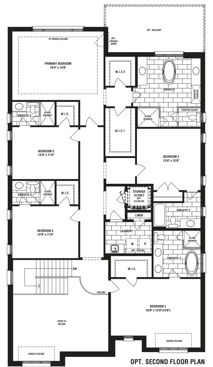
OPT. SECOND FLOOR PLAN ELEV. 'A' W/ 5 BEDROOM
