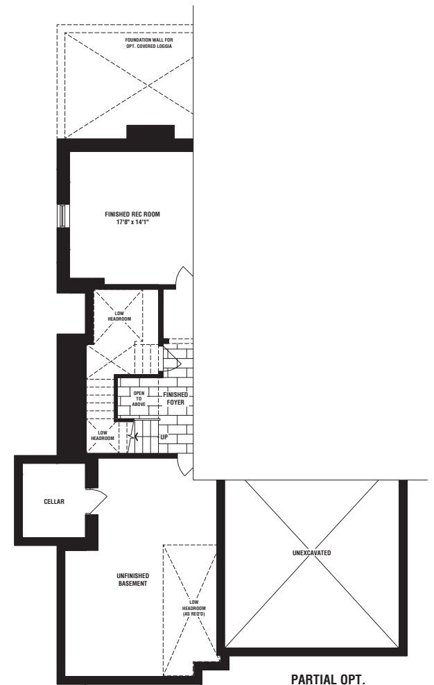
PARTIAL OPT. FINISHED BASEMENT PLAN ELEV. 'B'
