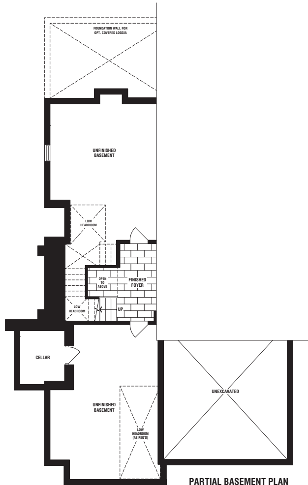
PARTIAL BASEMENT PLAN ELEV. 'C'
