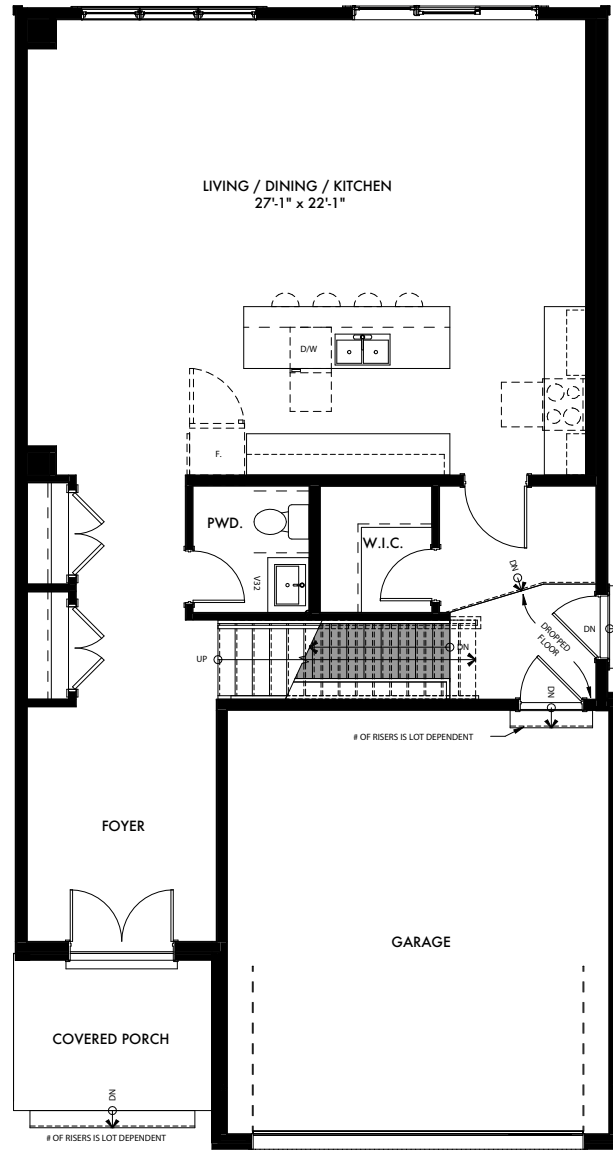
MAIN FLOOR 1105 SQ FT
