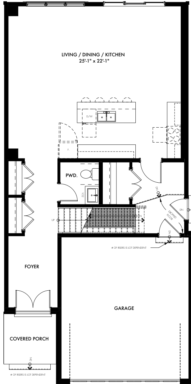
MAIN FLOOR 1003 SQ FT
