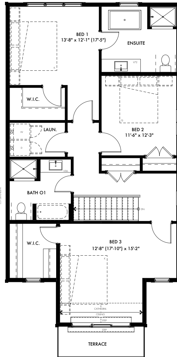
SECOND FLOOR 1207 SQ FT
