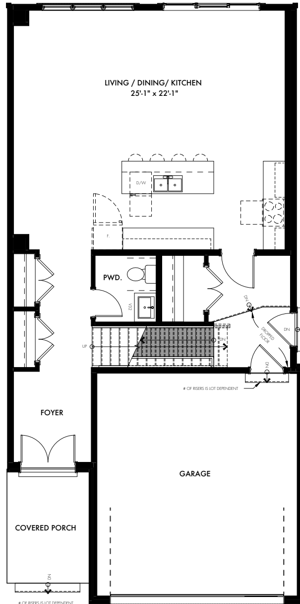
MAIN FLOOR 987 SQ FT
