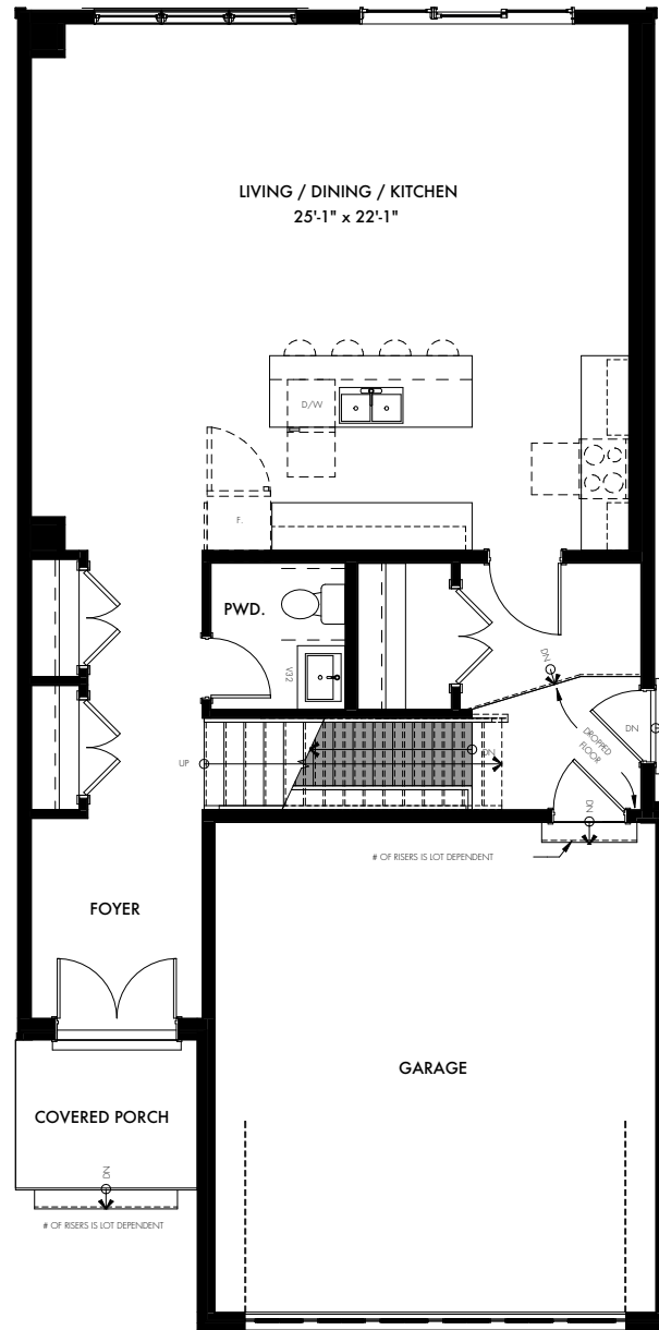
MAIN FLOOR 987 SQ FT
