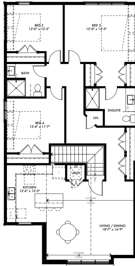
SECOND FLOOR OPT. B
