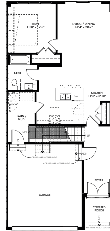
MAIN FLOOR 1022 SQ FT
