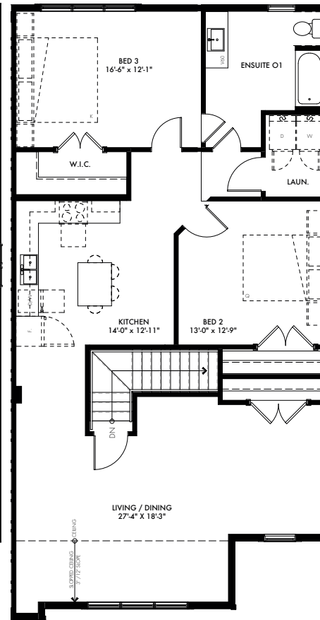
SECOND FLOOR 1418 SQ FT
