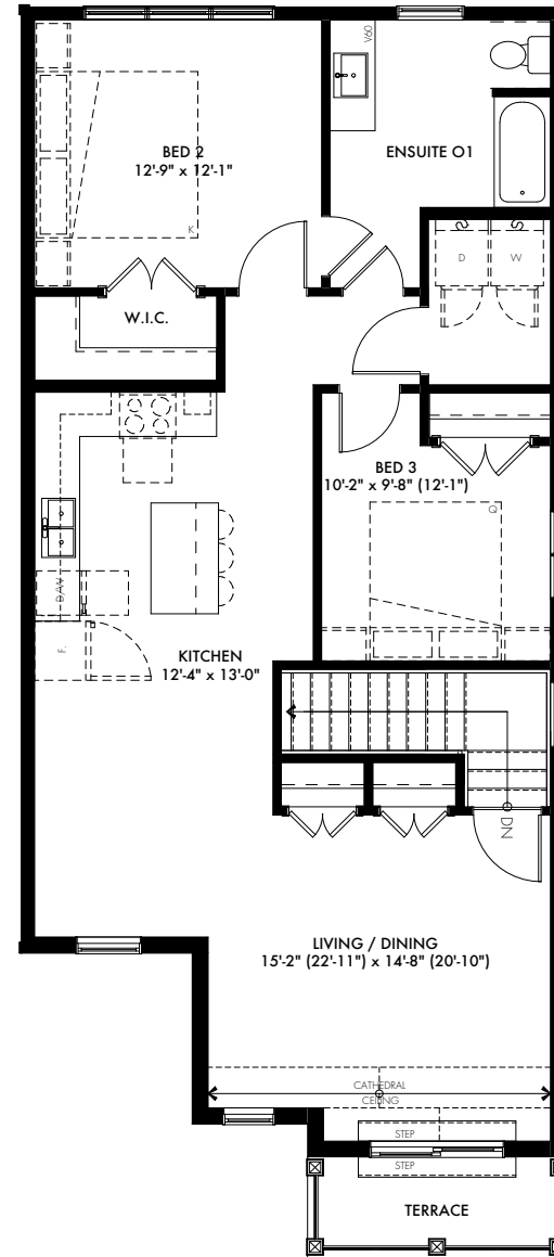
SECOND FLOOR 1131 SQ FT
