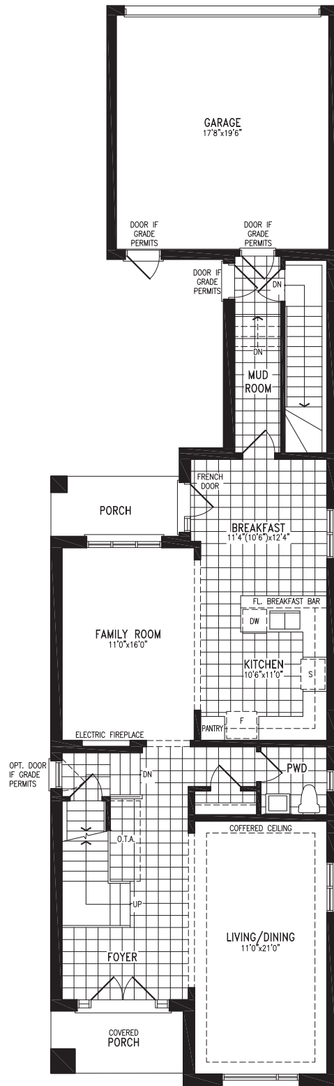
Elevation C GROUND FLOOR
