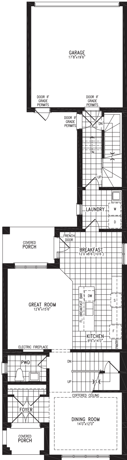
Elevation B GROUND FLOOR
