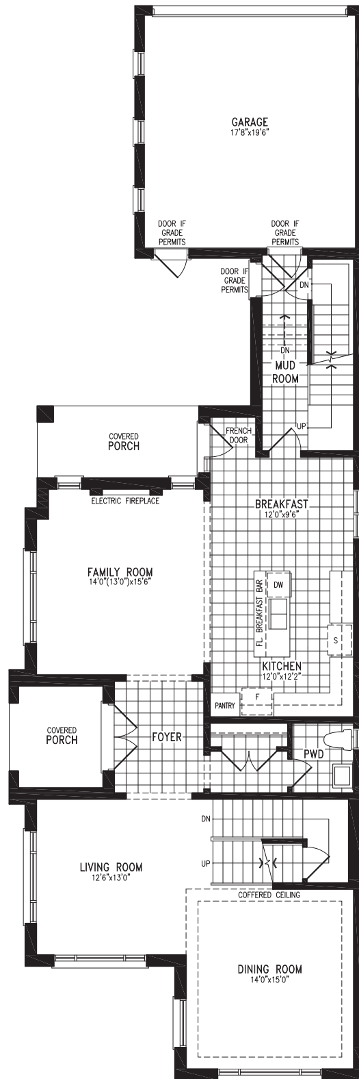
Elevation C GROUND FLOOR
