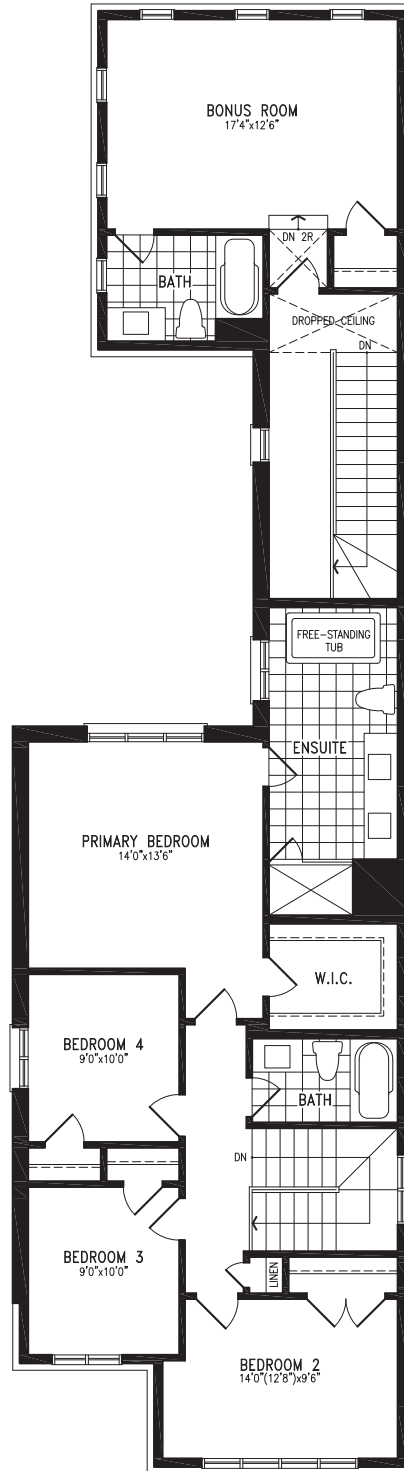
Elevation A SECOND FLOOR
