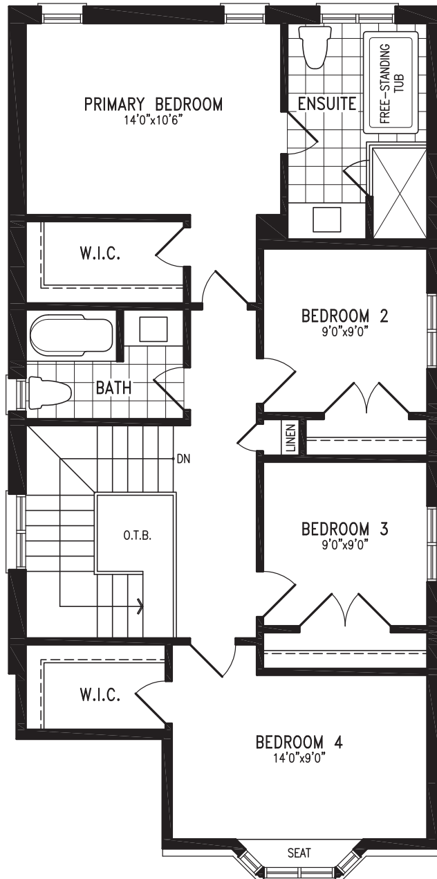
Elevation B SECOND FLOOR
