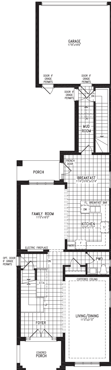
Elevation B GROUND FLOOR
