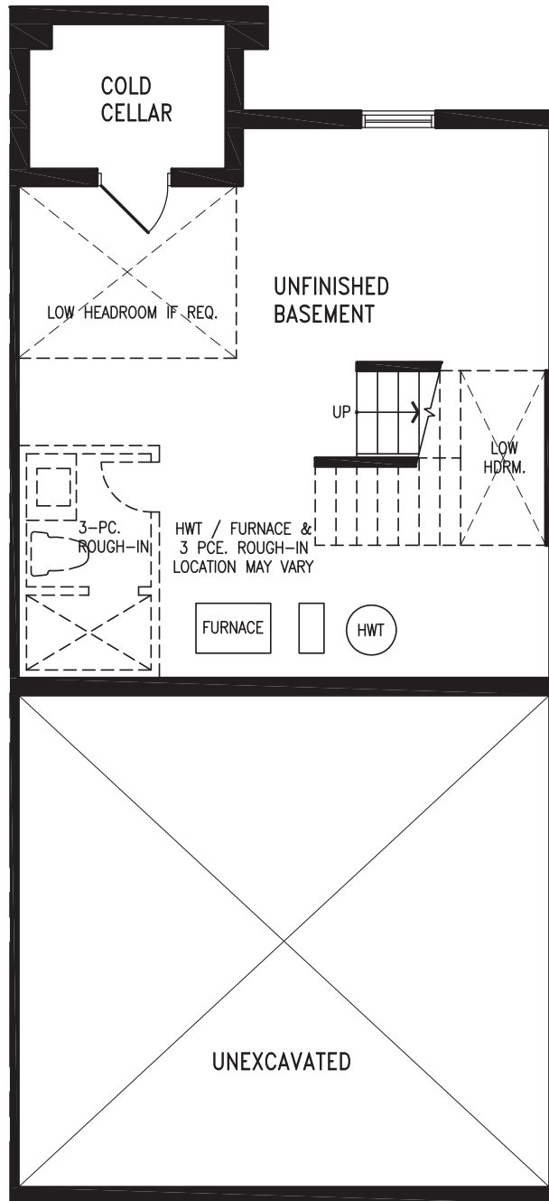
Elevation A BASEMENT
