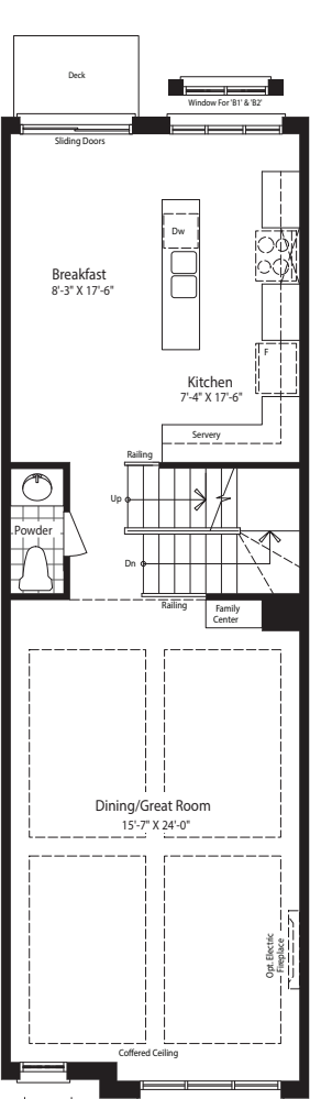
Alt. 1 Main Floor Plan Elevation 'A1' & 'A2' W/ Upper Floor Laundry
