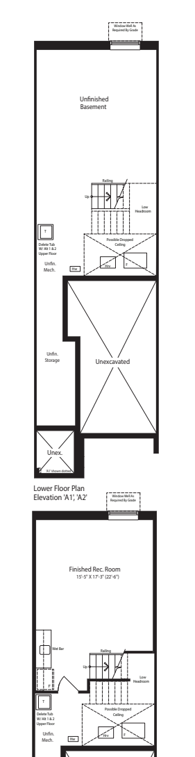
Opt. Finished Lower Floor Plan Elevation 'A1' & 'A2' Only available at time of structural Décor appointment
