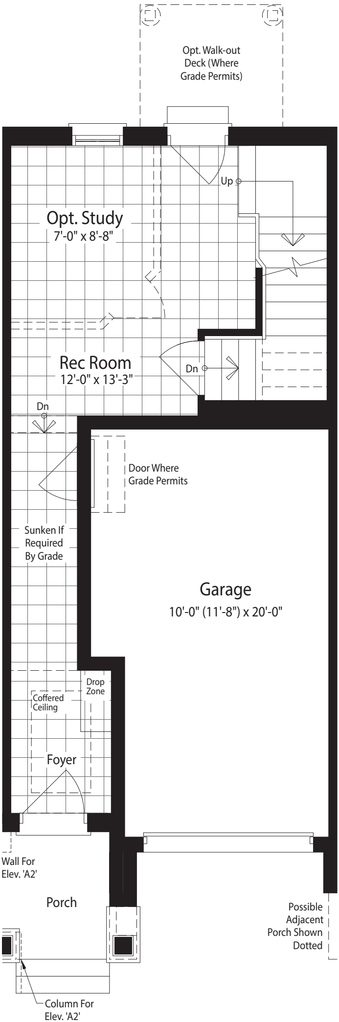
Ground Floor Plan Elevation 'A1', 'A2'
