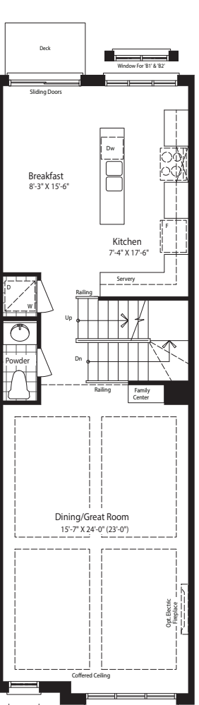
Alt. 1 Main Floor Plan Elevation 'A1' & 'A2'
