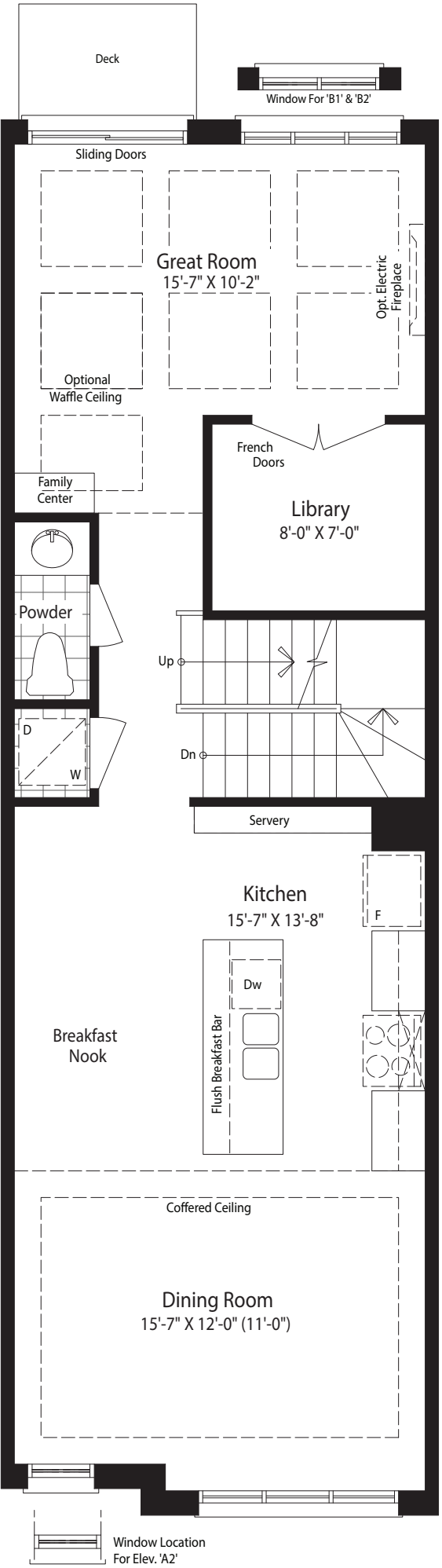
Main Floor Plan Elevation 'A1' & 'A2'
