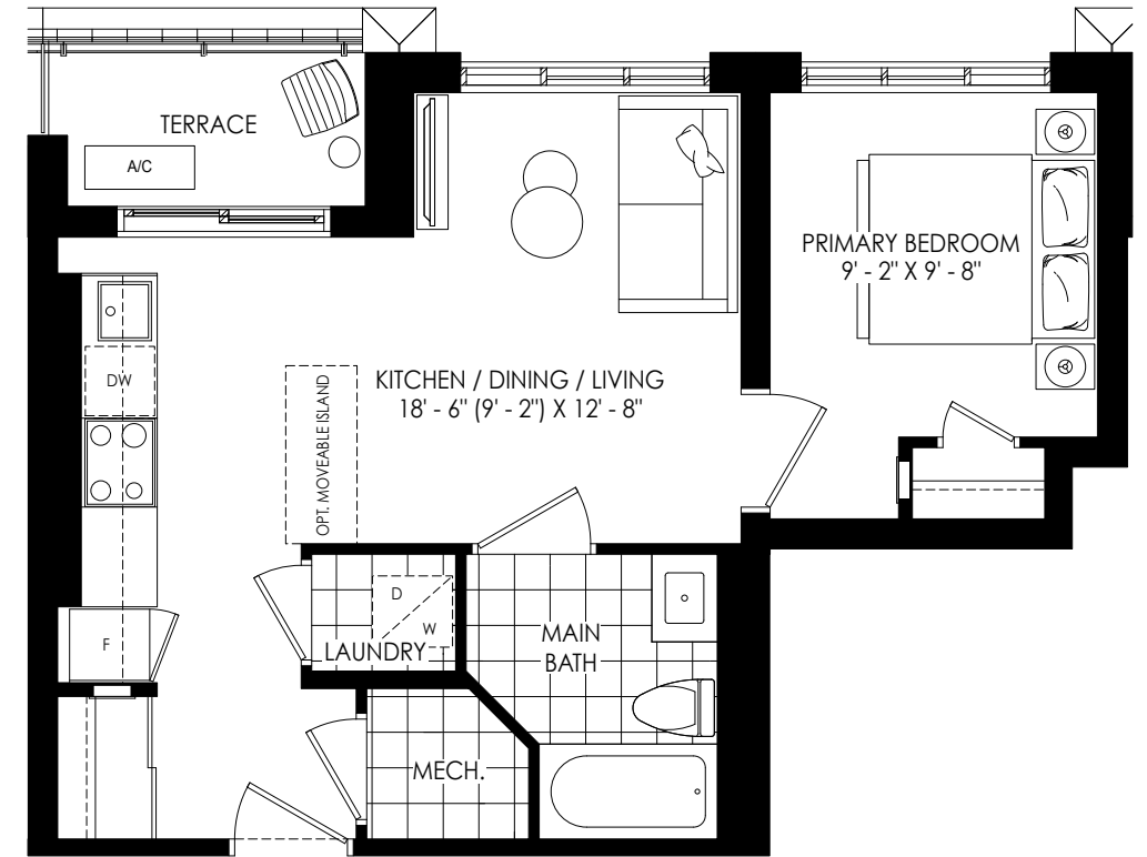
THIRD FLOOR
