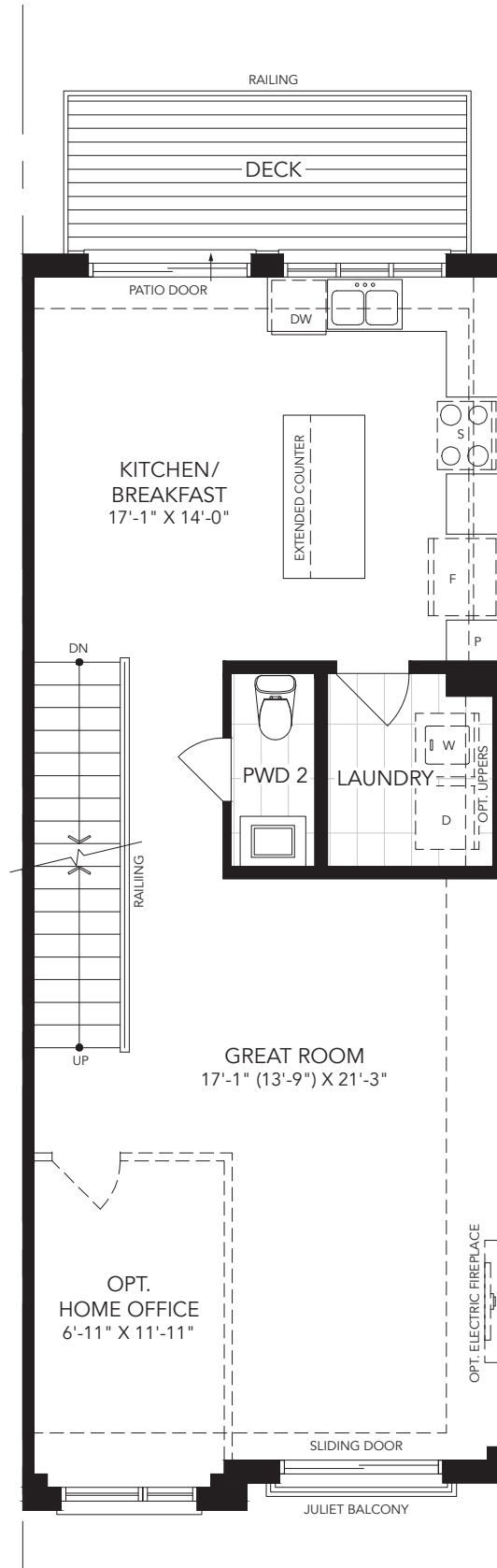
MAIN FLOOR PLAN A
