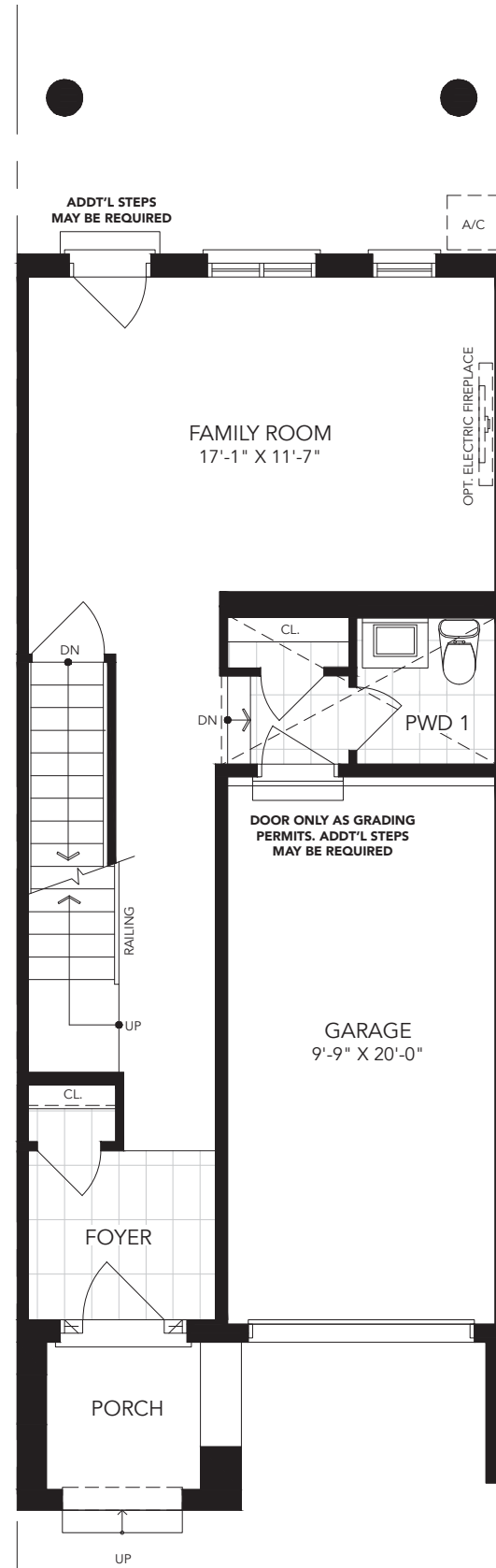
GROUND FLOOR PLAN A
