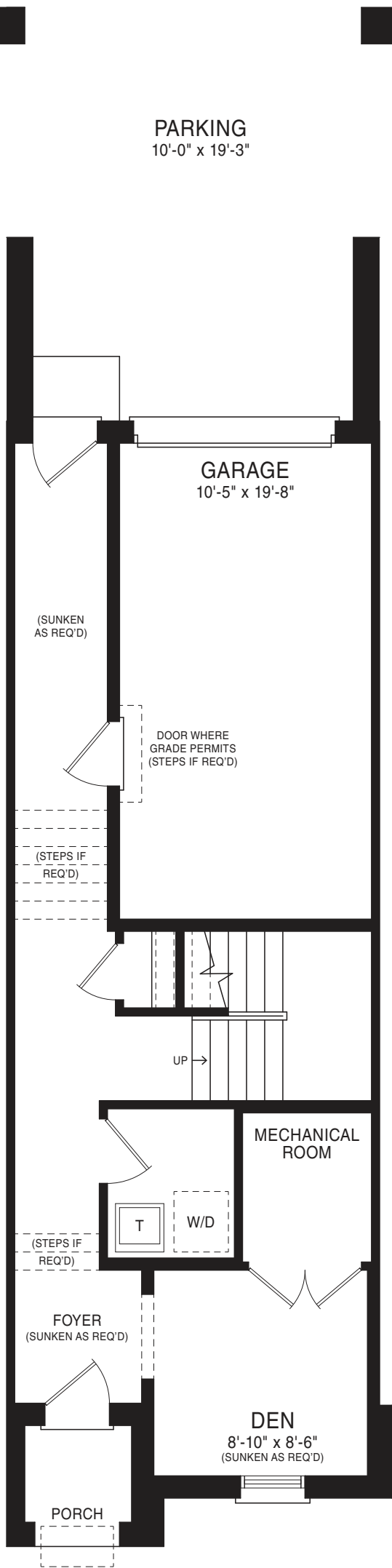
LOWER FLOOR PLAN STYLE D
