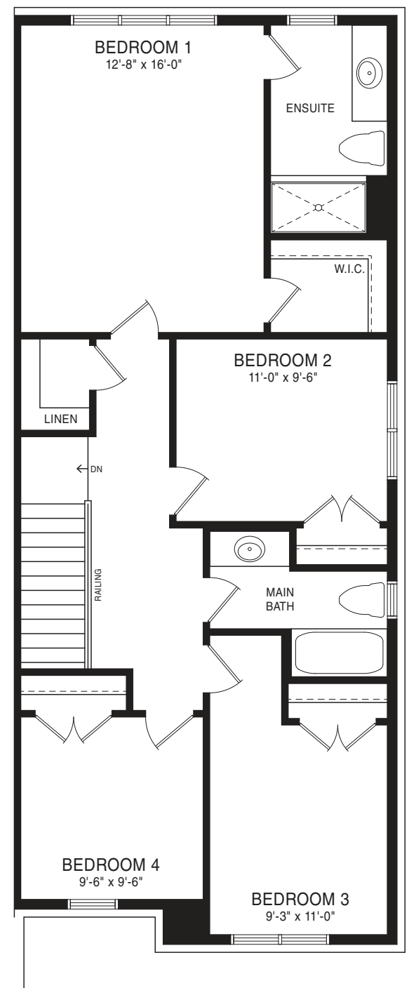
UPPER FLOOR PLAN STYLE D
