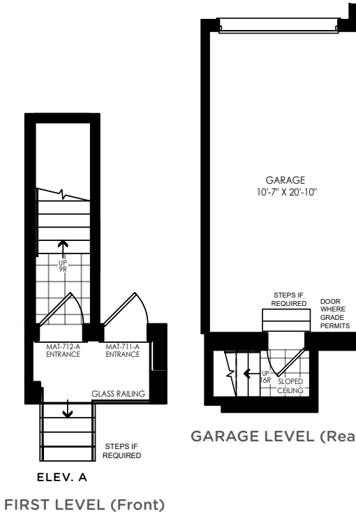
FIRST LEVEL (Front)
