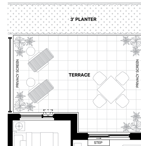
Level 2 Suite Area: 493 sq. ft. Outdoor Area: 283 sq. ft. Total Area: 776 sq. ft.
