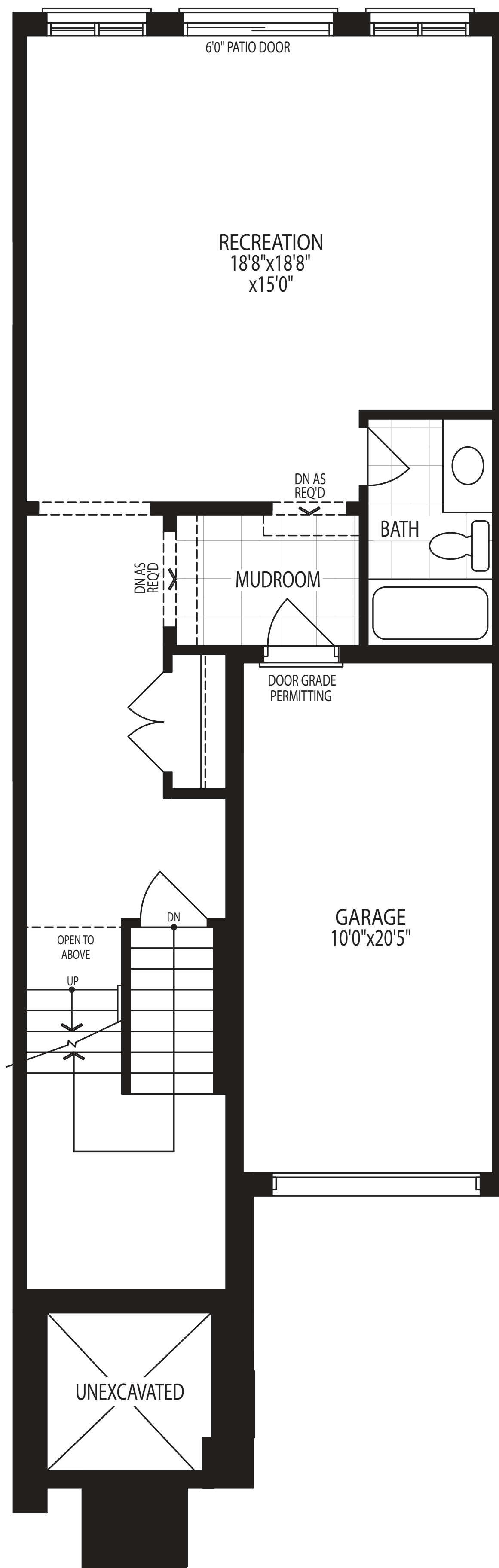
GROUND FLOOR PLAN ELEV. A
