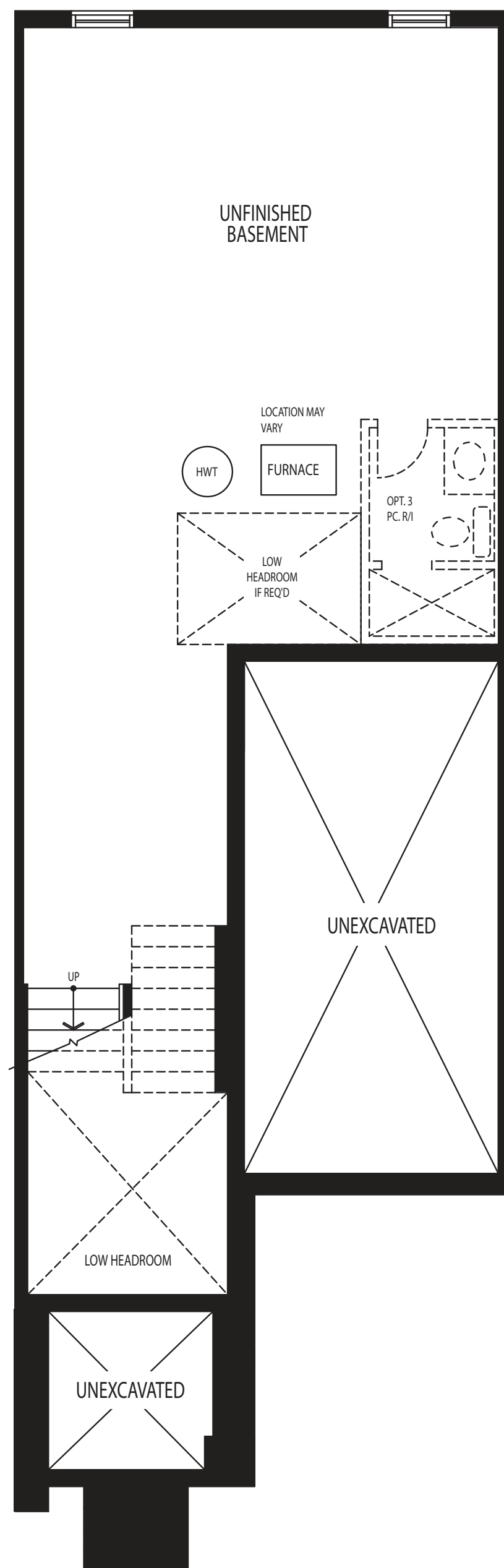
BASEMENT PLAN ELEV. A
