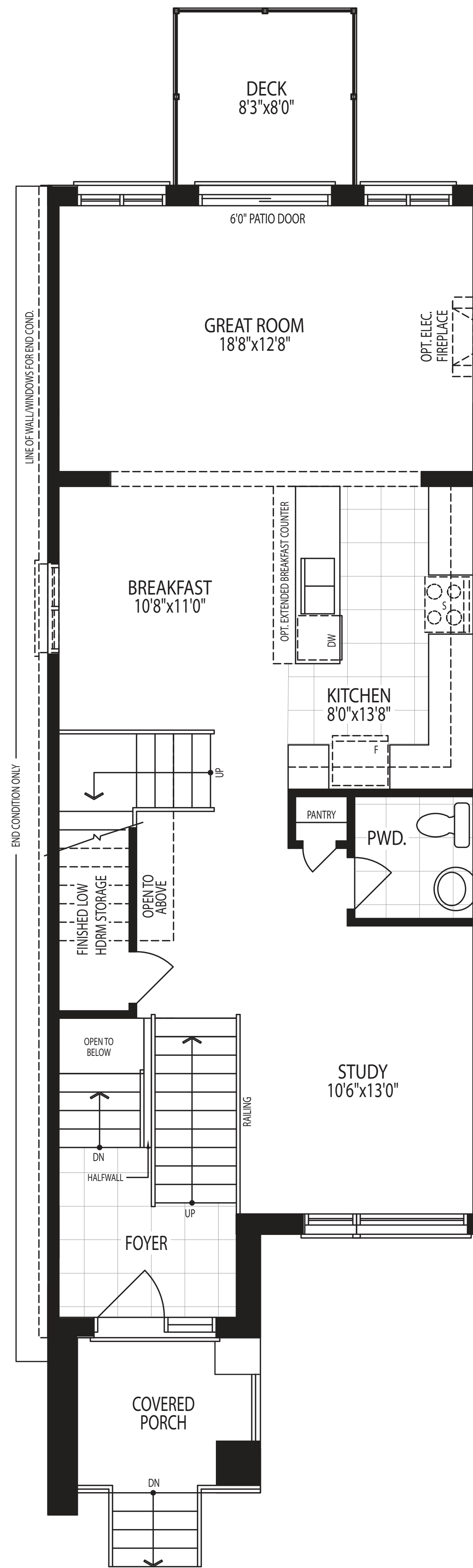
MAIN FLOOR PLAN ELEV. A
