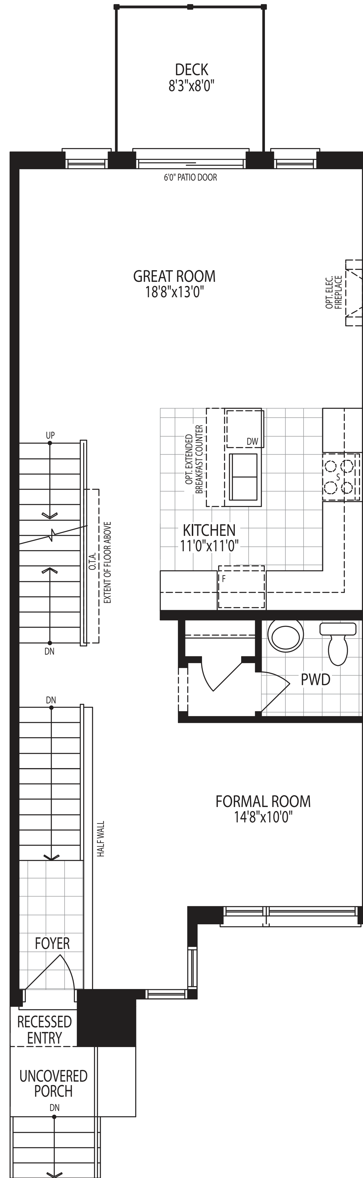
MAIN FLOOR PLAN ELEV. D
