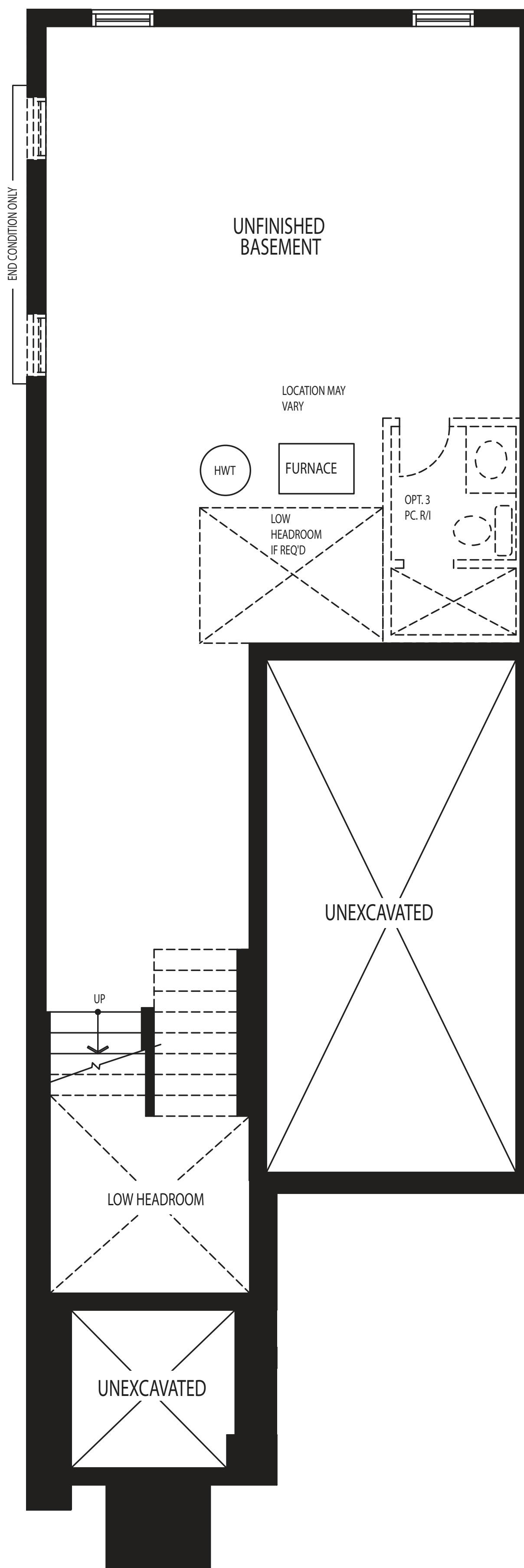
BASEMENT PLAN ELEV. A
