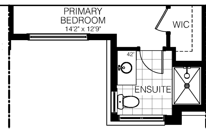
SECOND FLOOR ELEV. M2
