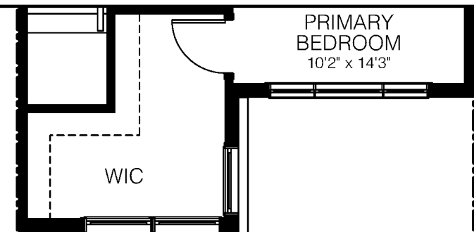
SECOND FLOOR ELEV. M1
