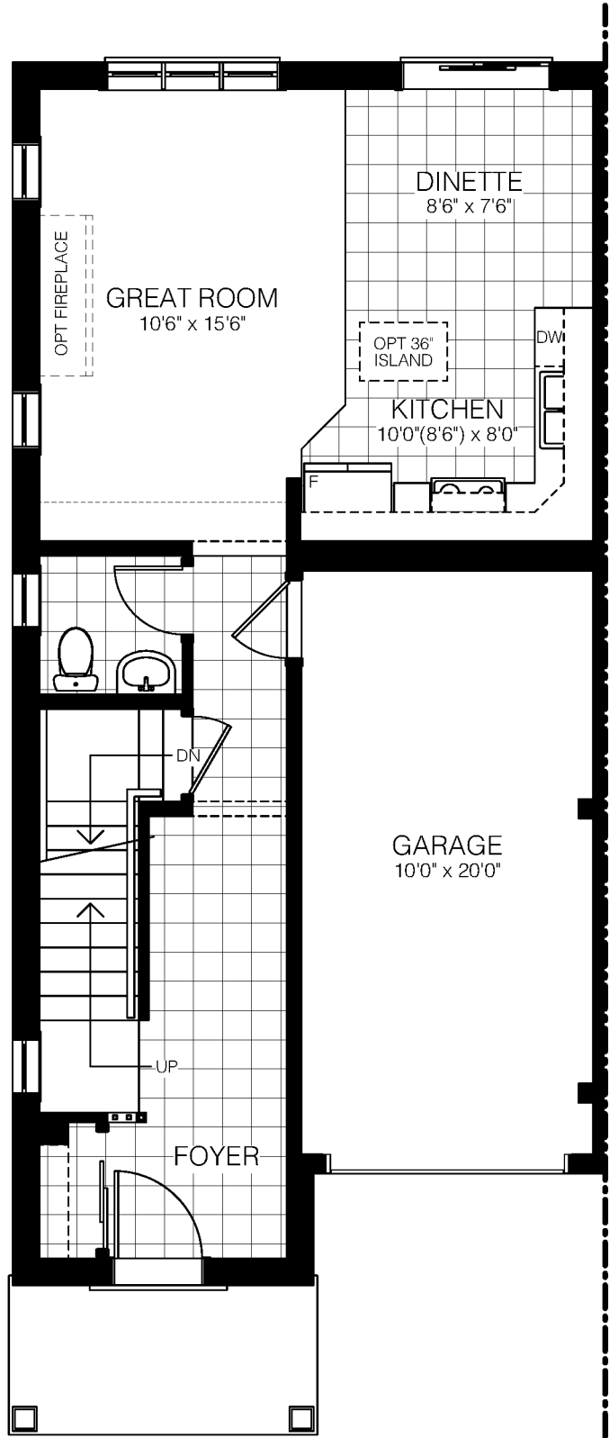
MAIN FLOOR ELEV. A
