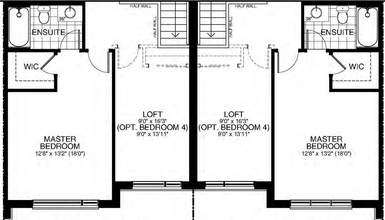
SECOND FLOOR ELEV. M3
