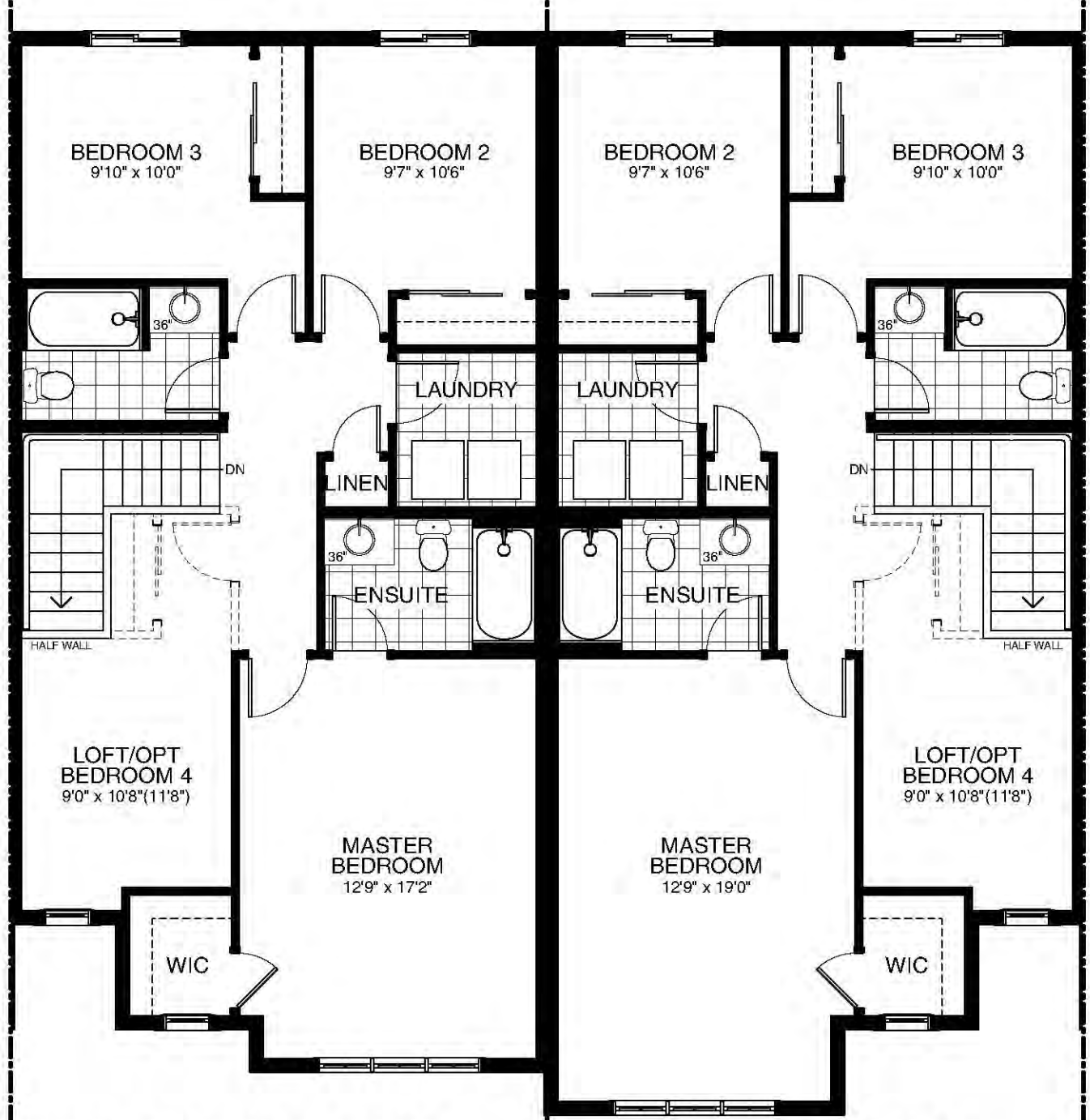
SECOND FLOOR ELEV. B1
