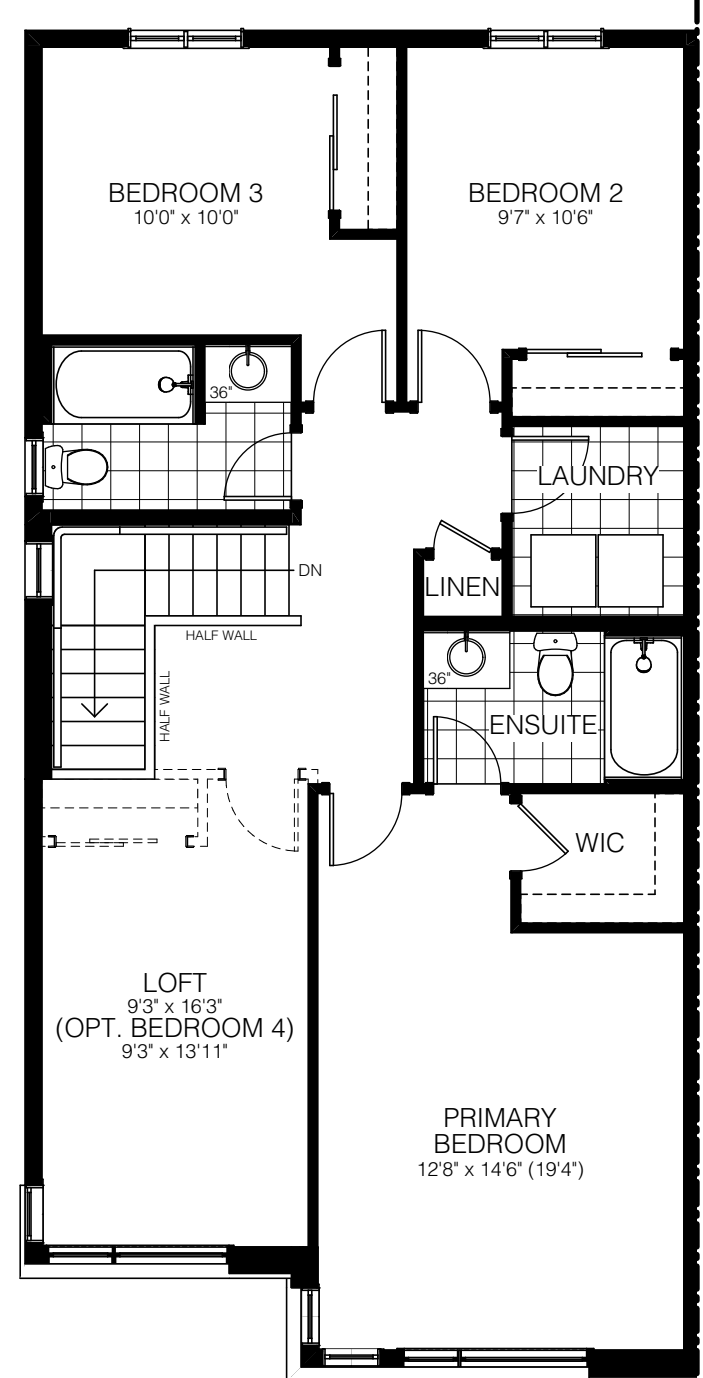
SECOND FLOOR ELEV. M3
