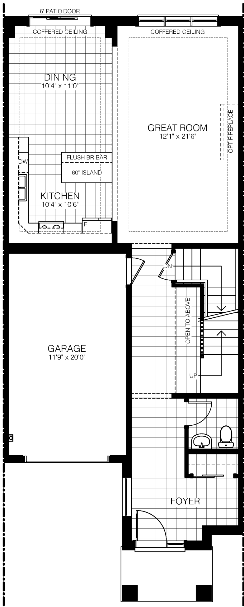
MAIN FLOOR ELEV. M1/M2
