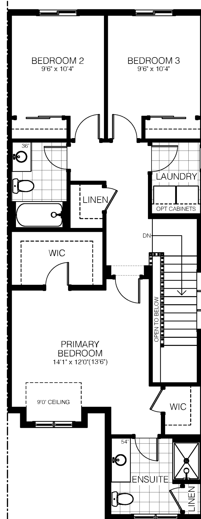
SECOND FLOOR ELEV. A
