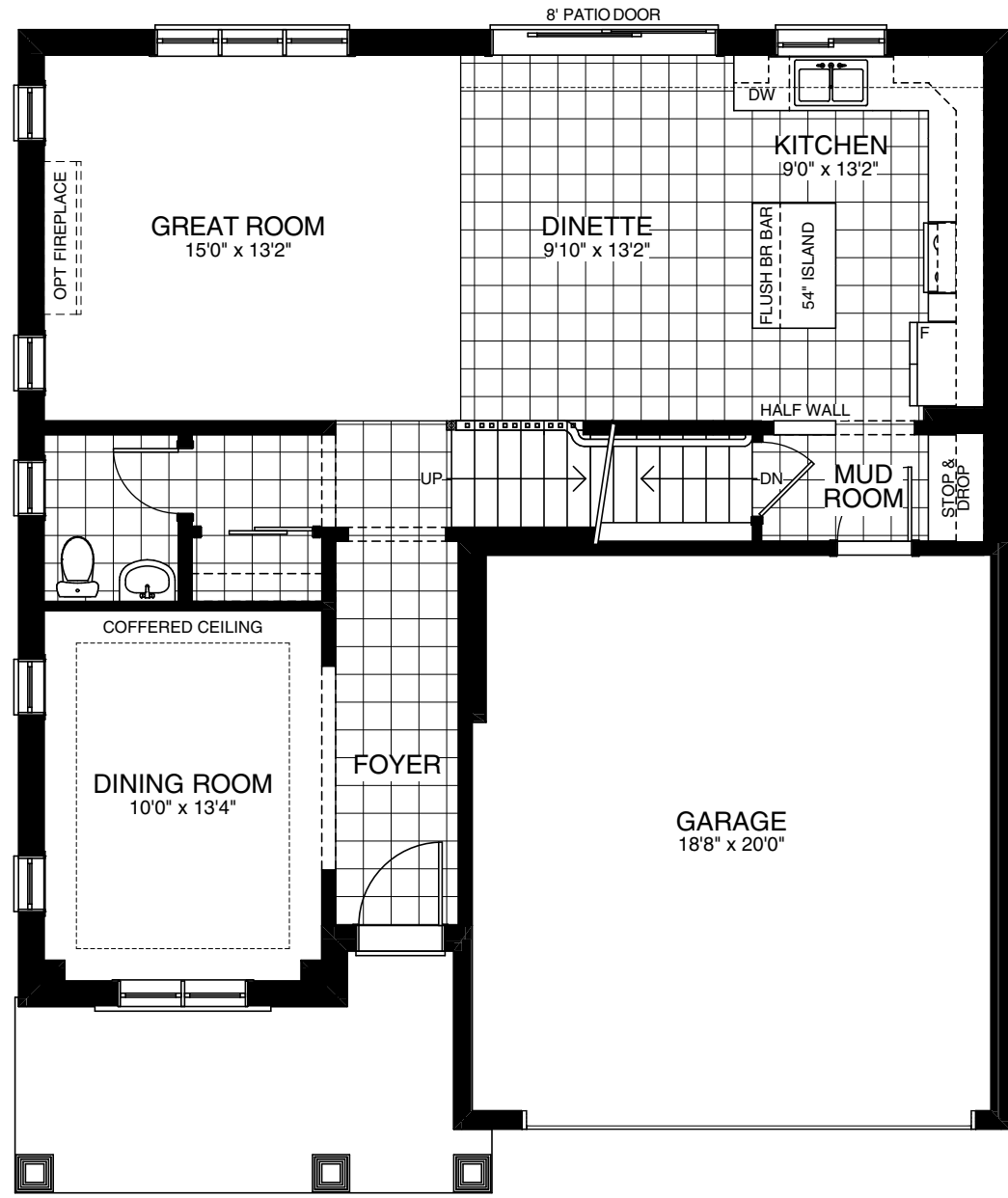
MAIN FLOOR ELEV. A
