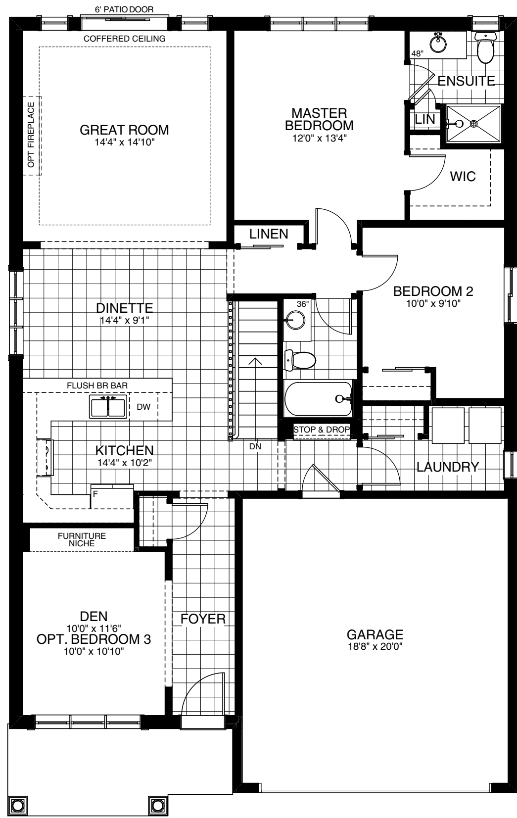
MAIN FLOOR ELEV. A
