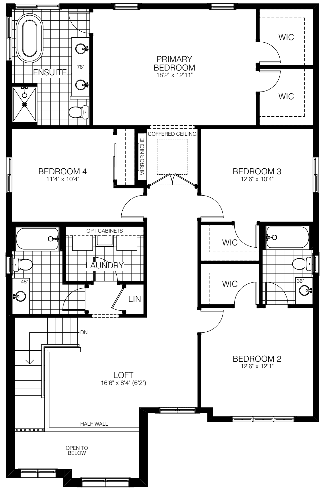
SECOND FLOOR ELEV. A 65 sq.ft. OPEN TO BELOW
