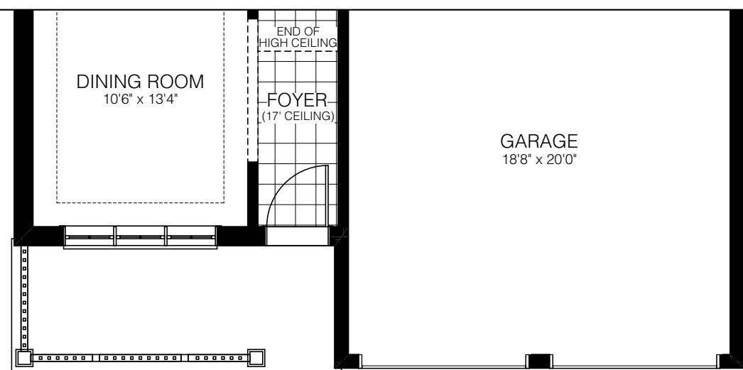
MAIN FLOOR ELEV. B
