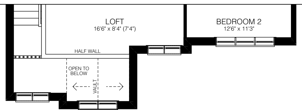
SECOND FLOOR ELEV. B 65 sq.ft. OPEN TO BELOW
