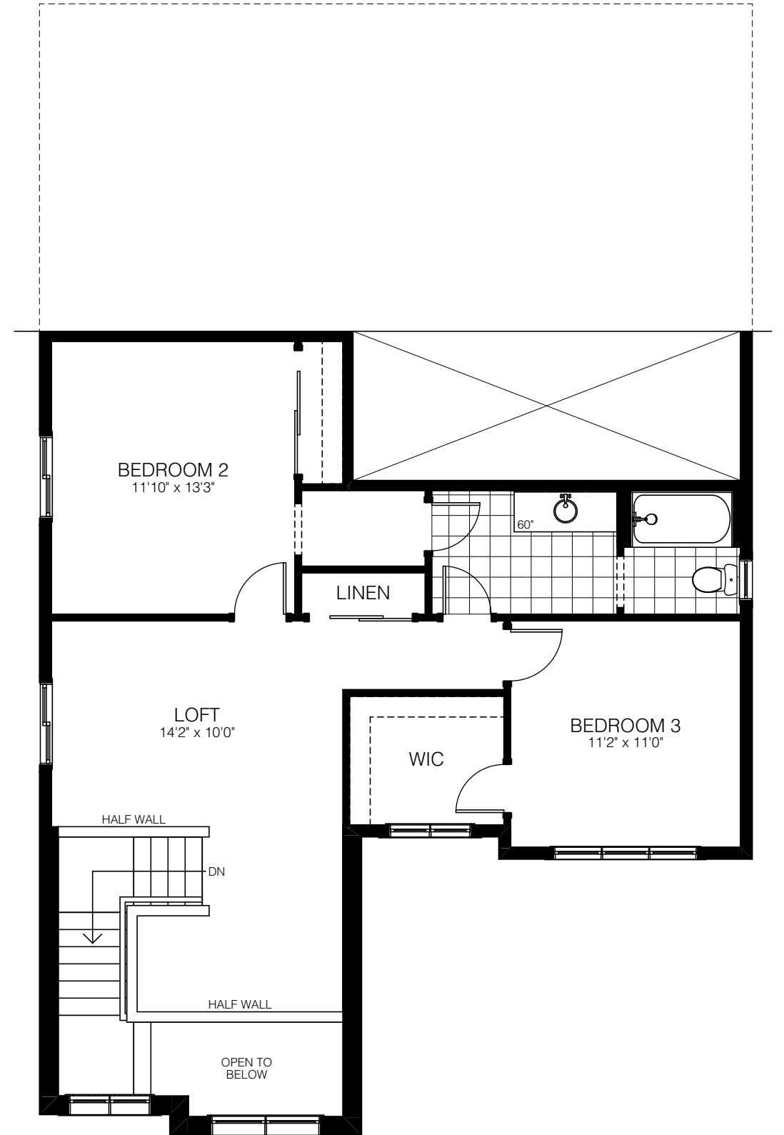
SECOND FLOOR ELEV. A 41 sq.ft. OPEN TO BELOW
