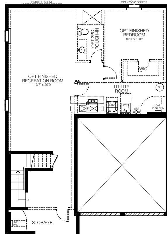
BASEMENT ELEV. A
