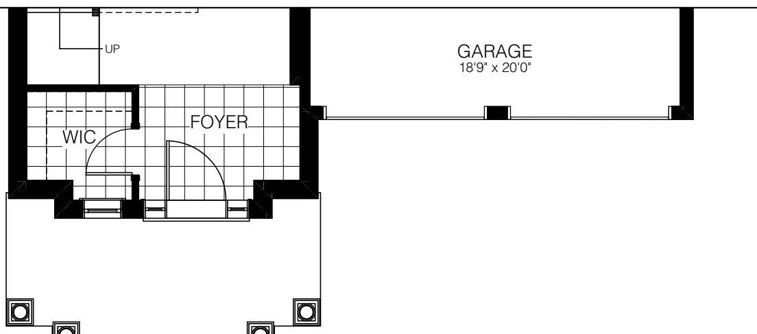
MAIN FLOOR ELEV. B
