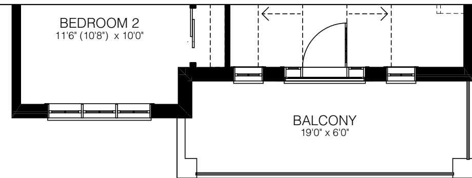
SECOND FLOOR ELEV. B 16 sq.ft. OPEN TO BELOW
