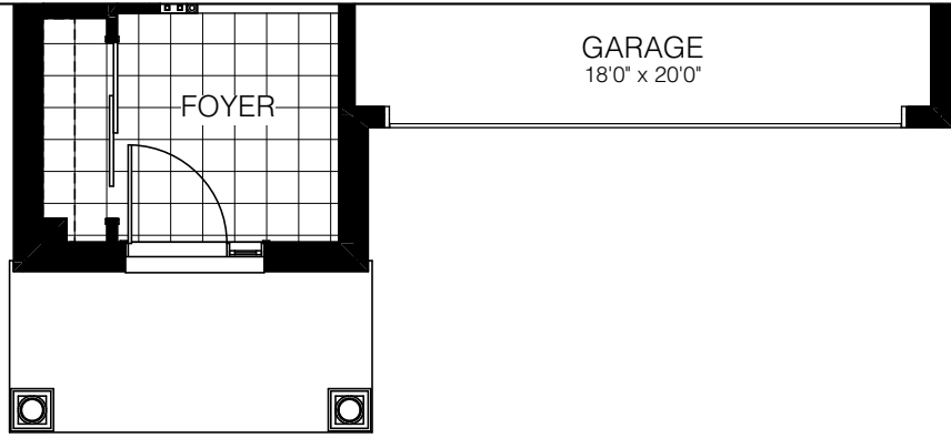
MAIN FLOOR ELEV. B
