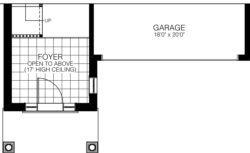
MAIN FLOOR ELEV. B
